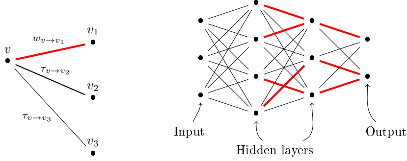
Figure 1: Left: The outward edges of a hidden neuron v and their weights. In this example, v_1 = s_{\max}^\theta(v) , so the weight of the edge in red, v \rightarrow v_1 , has its value fixed as w_{v \rightarrow v_1} . The weights of the remaining edges, \tau_{v \rightarrow v_2} and \tau_{v \rightarrow v_3} , are free to vary. Right: In red, all the edges whose weights are fixed. The remaining edges, in black, constitute the set F_\theta .
