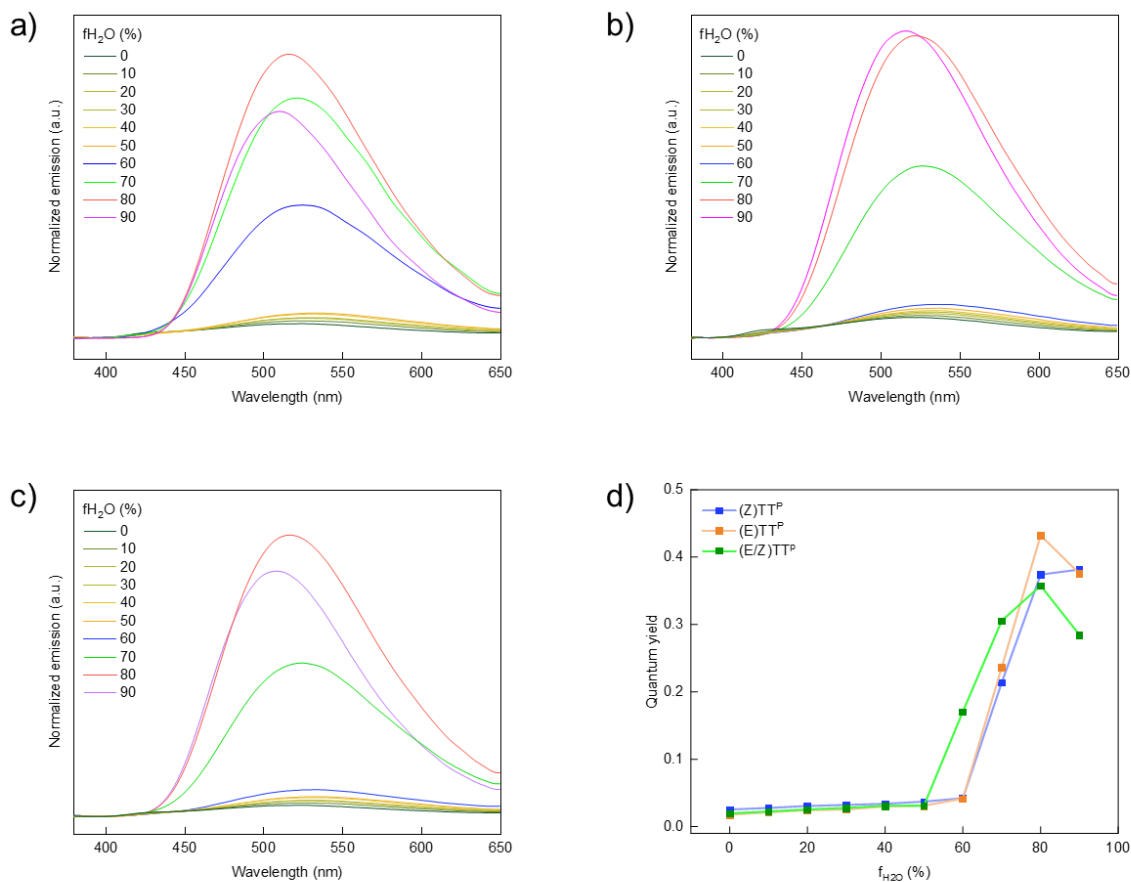
Figure 3. Emission of a) the isomers mixture, b) the Z-isomer and c) the E-isomer of TT P (n=16) in various water/DMSO mixtures. d) Evolution of the fluorescence quantum efficiency of the isomers mixture (green), (Z) isomer (blue) and (E) isomer (orange) of TT P in various water/DMSO mixtures.
