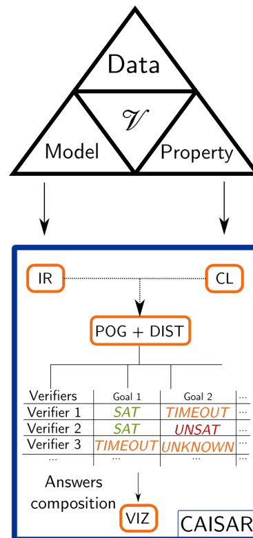
Figure 1: CAISAR overall architecture
