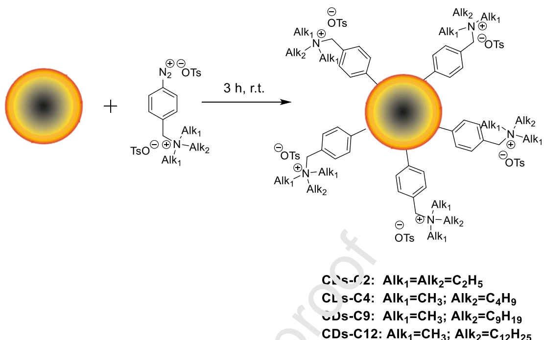
Figure 2. Preparation of CD-C2, CD-C4, CD-C9 and CD-C12.
