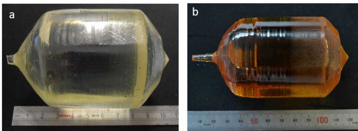
Figure 4. LGT bulk single crystals grown by using 1% \text{Ga}_2\text{O}_3 excess: (A) Argon growth atmosphere, (B) Argon +0.5% \text{O}_2
