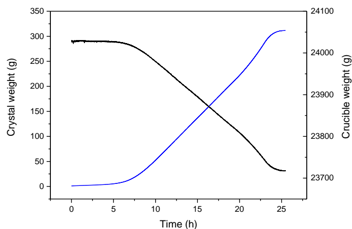
Figure 5. Evolution of the LGT mass and the crucible weight during LGT automatic growth using 1% \text{Ga}_2\text{O}_3 excess
