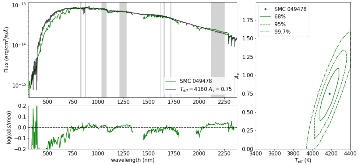
Figure A17. Same as Fig. A10 but for SMC 049478.
