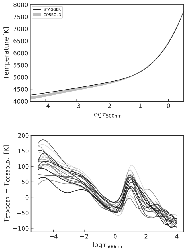
Fig. 1: Top panel : temperature structure of STAGGER and CO5BOLD model atmospheres. Gray area depicts variations among temporarily resolved snapshots in CO5BOLD simulations. Bottom panel : absolute difference in temperature structure of STAGGER and CO5BOLD model atmospheres. Each line corresponds to a temporarily resolved snapshot of CO5BOLD simulations. See Sect. 2.3 for details.
