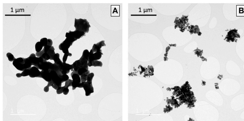
FIGURE 2 | TEM images of (A) AgNbO 3 and (B) Ag 0.70 La 0.10 □ 0.20 NbO 3 after annealing at 650°C showing the difference in particles size between unsubstituted and substituted oxides.
