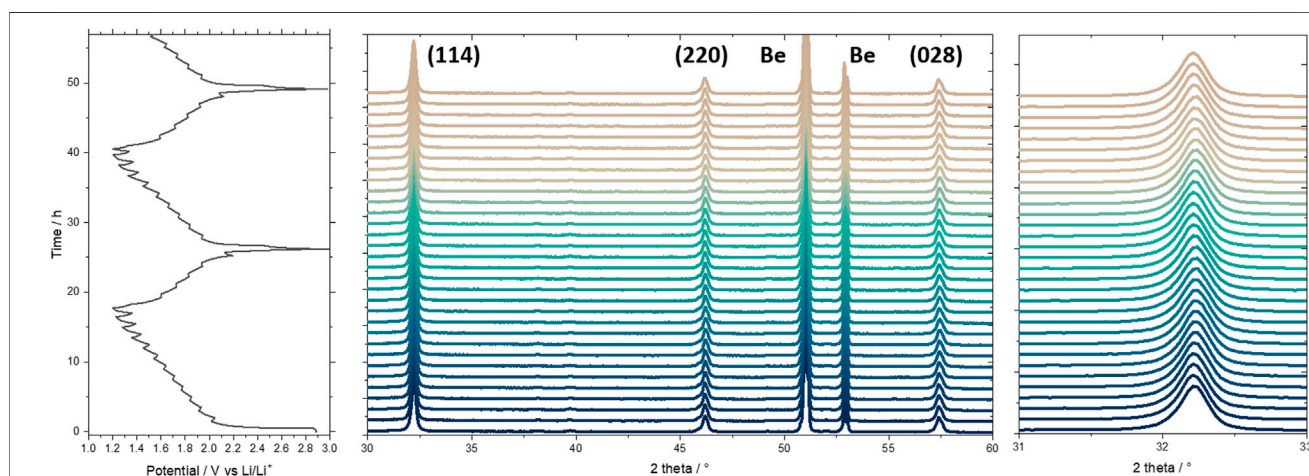
FIGURE 6 | In situ XRD patterns of the Ag 0.70 La 0.10 NbO 3 at a current of 0.02 A g -1 with corresponding voltage-time curve.
