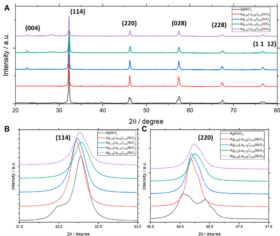
FIGURE 3 | (A–C) XRD patterns of Ag 1-3x La x □ 2x NbO 3 for different value of x.
