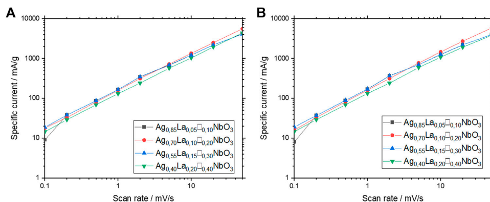
FIGURE 5 | (A) Linear regression from power law in the reduction peaks of Ag 1-3x La x NbO 3 for different value of x. (B) Linear regression from power law in the oxidation peaks of Ag 1-3x La x NbO 3 for different value of x.
