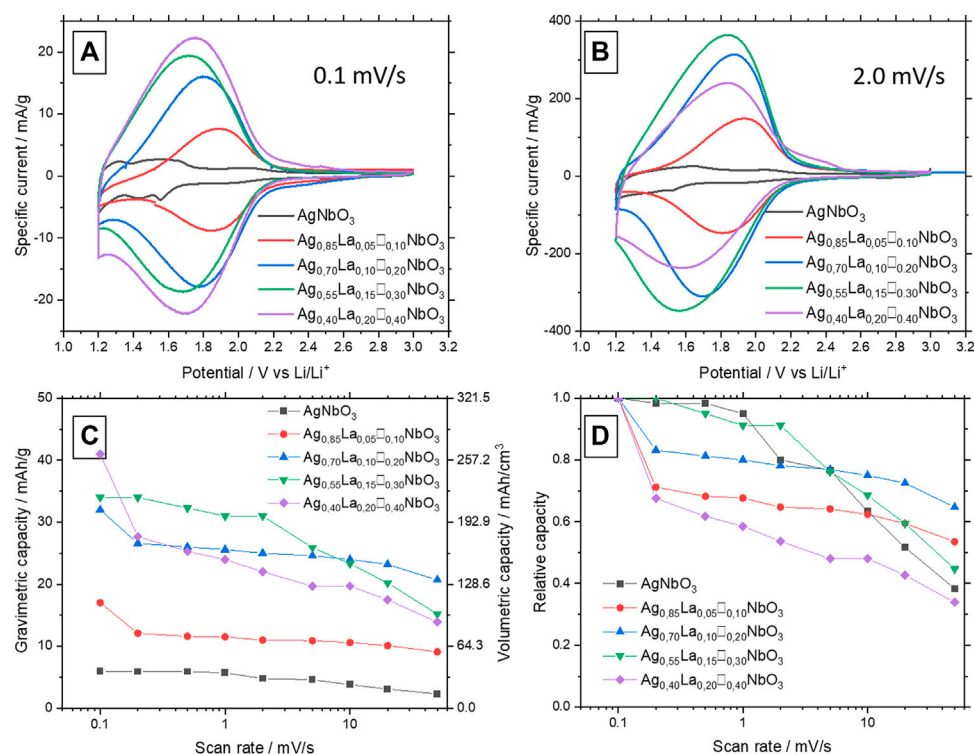
FIGURE 4 | (A) CV at 0.1 mV s -1 between 1.2 and 3 V of Ag 1-3x La x NbO 3 for different value of x. (B) CV at 2.0 mV s -1 between 1.2 and 3 V of Ag 1-3x La x NbO 3 for different value of x. (C) Specific capacity of Ag 1-3x La x NbO 3 for different value of x in function of the scan rate. (D) Relative capacity of Ag 1-3x La x NbO 3 for different value of x in function of the scan rate.
