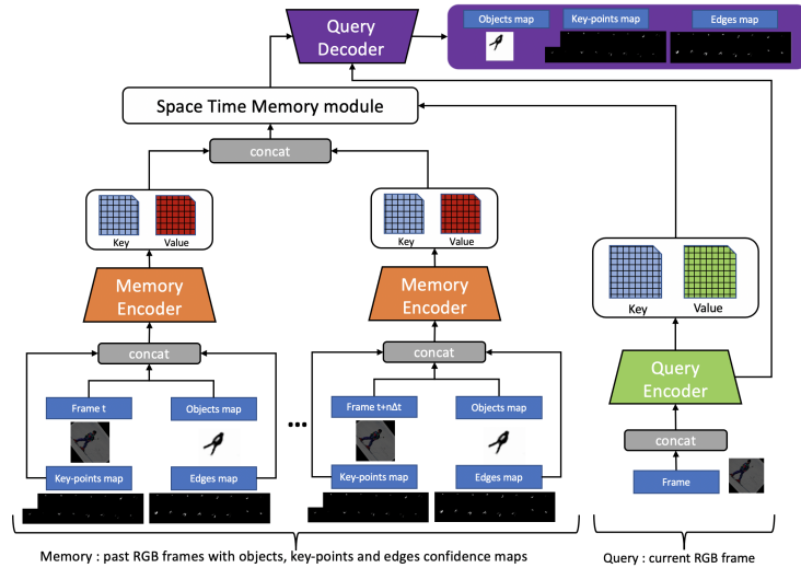
Fig. 2. Our proposed STM-skeletons architecture.
