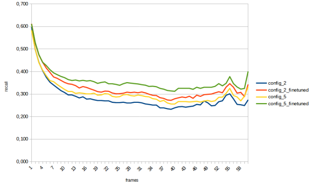
Fig. 7. Evolution of recall over time depending on model training configuration.
