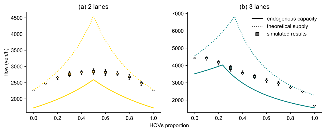
Figure 3: Comparing the model with the theoretical supply and simulation results for (a) two upstream lanes and (b) three upstream lanes
