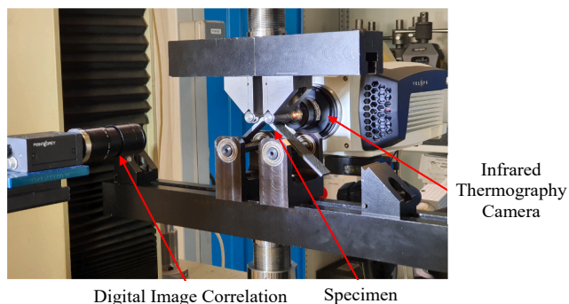
Fig. 6. Setup of the four-point bending test. (For interpretation of the references to colour in this figure legend, the reader is referred to the web version of this article.)
