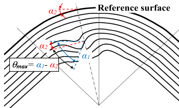
Fig. 7. Measure of the maximum misalignment angle. (For interpretation of the references to colour in this figure legend, the reader is referred to the web version of this article.)
