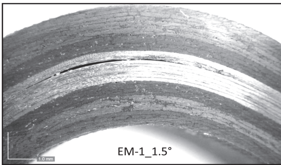
Fig. 17. Example of EM-1 specimen with presence of initial delamination.
