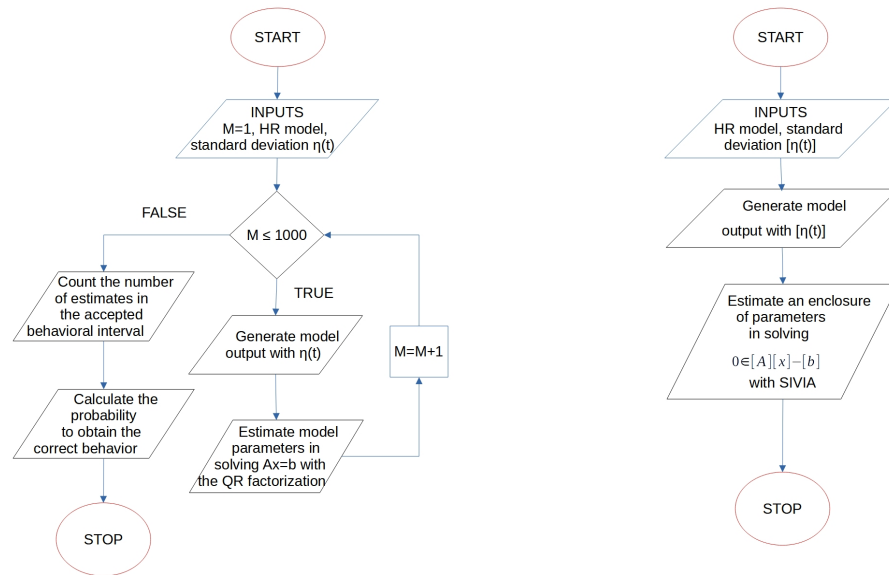
(a) (b) Figure 2. These two diagrams summarize the differences between the procedure presented in [5] and the one presented in this paper. (a) Diagram summarizing the stochastic procedure, presented in [5]. (b) Diagram summarizing the interval procedure, presented in this paper.
