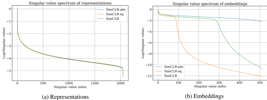
Figure S3: Singular value distribution of the embeddings and representations computed on the training set of ImageNet for SimCLR, SimCLR-abs and SimCLR-sq. All methods use 512 dimensional embeddings.
