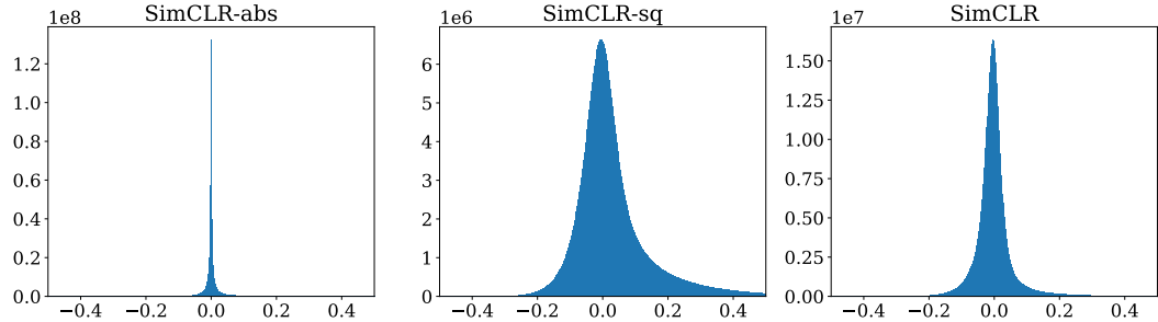
Figure S2: Histogram of cosine similarities for negative pairs in SimCLR-abs, SimCLR-sq and SimCLR.
