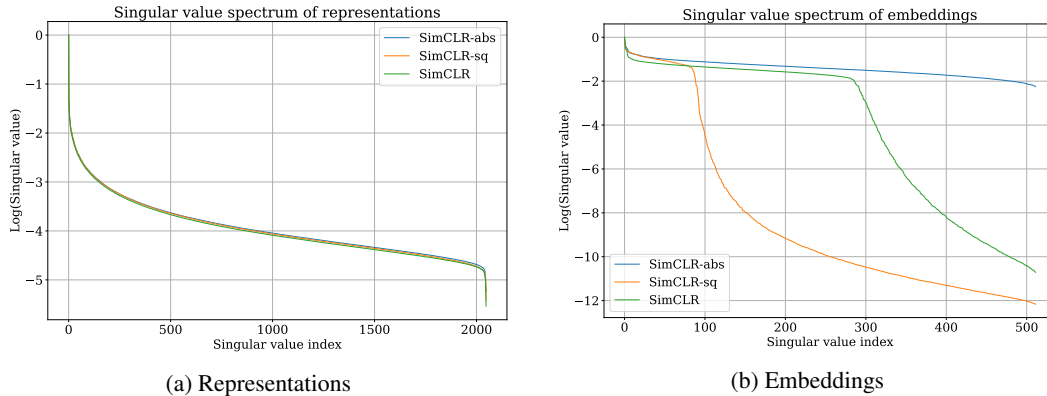
Figure S3: Singular value distribution of the embeddings and representations computed on the training set of ImageNet for SimCLR, SimCLR-abs and SimCLR-sq. All methods use 512 dimensional embeddings.
