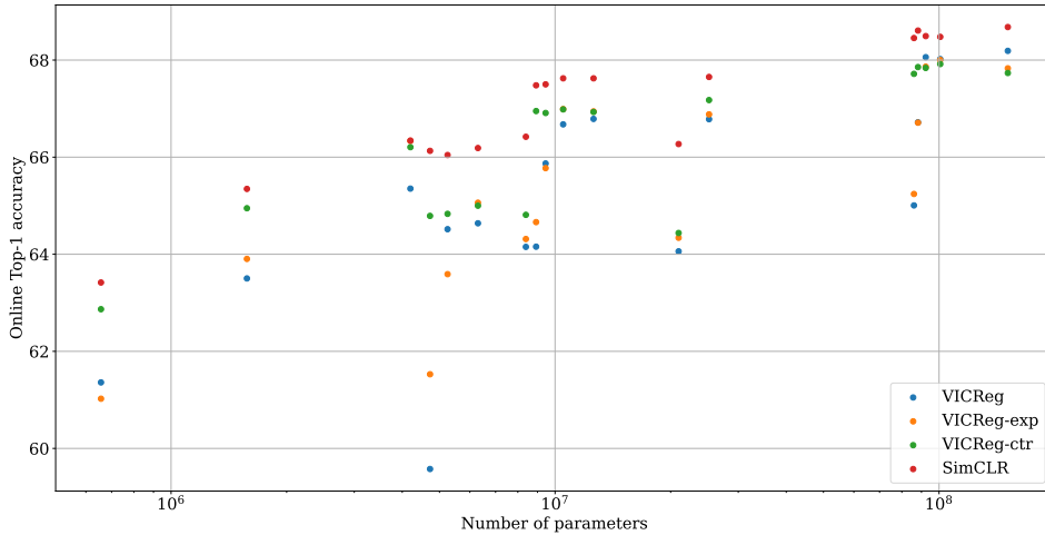
Figure S5: Online performance on ImageNet for VICReg, VICReg-exp, VICReg-ctr, and SimCLR with respect to the number of parameters in their projector.
