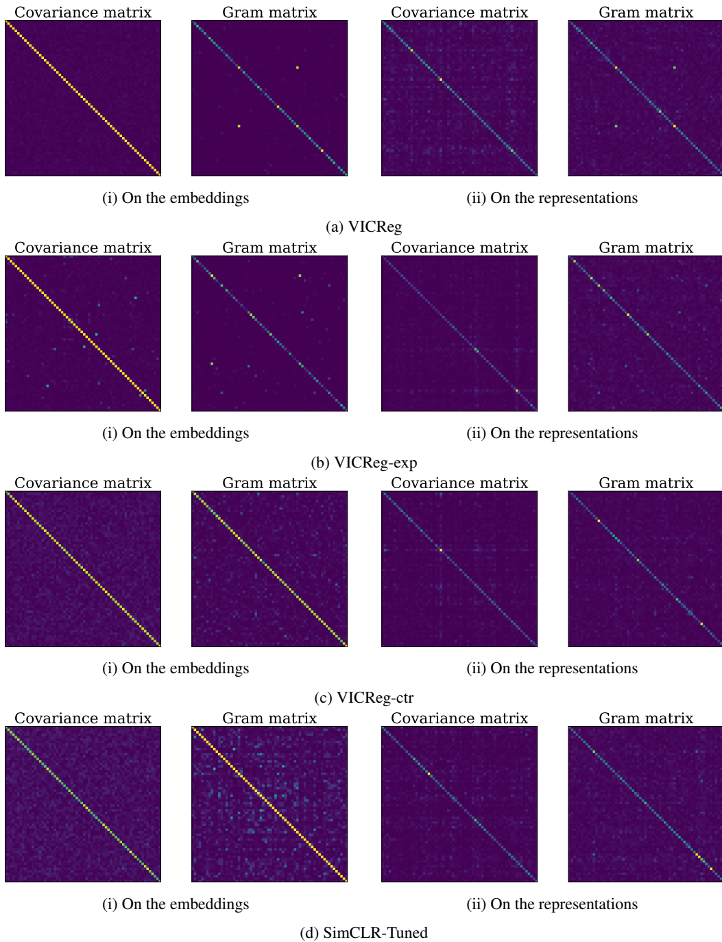
Figure S6: Covariance and similarity matrices on a random part of the ImageNet training set, using VICReg, VICReg-exp, VICReg-ctr, and SimCLR pretrained on ImageNet for 100 epochs. The covariance matrix is limited to the first 64 dimensions, while the Gram matrix is limited to the first 64 samples. In all cases, we used a projector with an output dimension of 2048, the same as the representation dimension.
