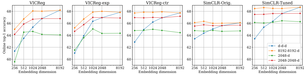
Figure S4: Online performance on ImageNet for VICReg, VICReg-exp, VICReg-ctr, and SimCLR with respect to embedding dimensions when changing the projector’s architecture.
