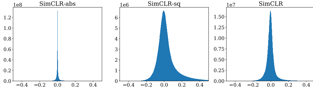
Figure S2: Histogram of cosine similarities for negative pairs in SimCLR-abs, SimCLR-sq and SimCLR.
