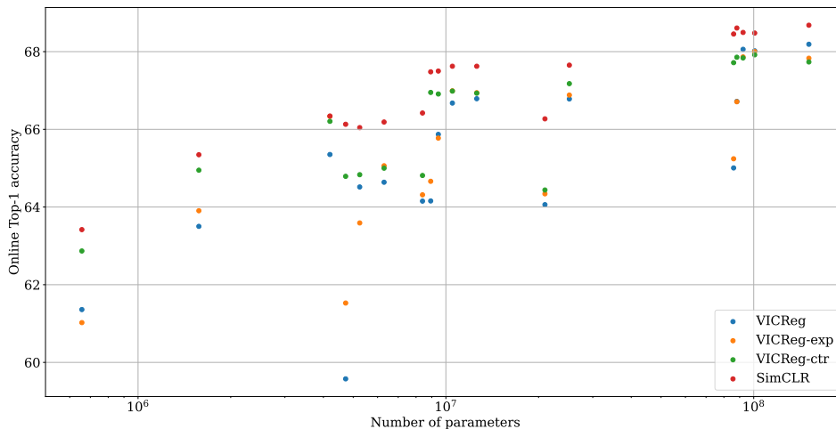
Figure S7: Online performance on ImageNet for VICReg, VICReg-exp, VICReg-ctr, and SimCLR with respect to the number of parameters in their projector.
