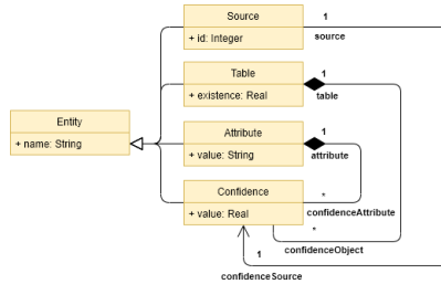
Figure 7: Confidences viewpoint
