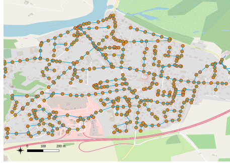
Figure 1: Example of spatial representation of sewerage networks
