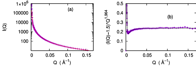
Fig. 2. (a) Plot of the observed intensity after circular averaging of the pattern of Figure 1 . The fit to equation (8) is shown (red line) (b) same plot after subtracting 1.5 and rescaling by Q^{1.964} , demonstrating the critical scattering.
