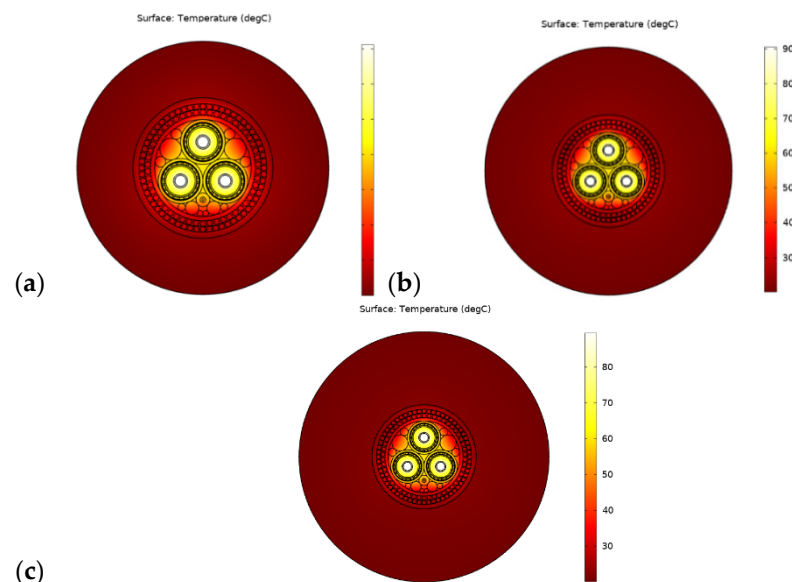
Figure 15. Steady-state temperature (°C) distribution for different ages of mussels (a) Juvenile, (b) Mix (c) Adult.
