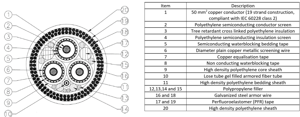
Figure 12. Cross section of a three phases DSEC.
