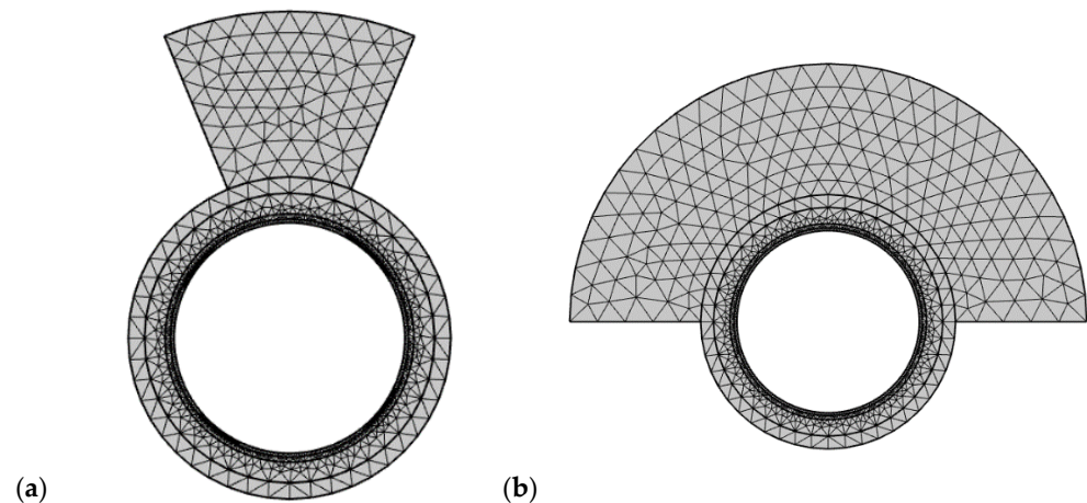
Figure 11. Fine mesh in COMSOL for (a) 25% (b) 50% mussel colonization.
