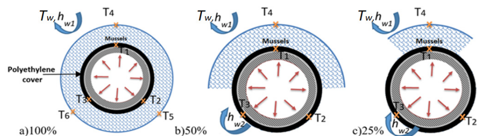
Figure 10. Various colonization distribution configurations around the heated covered polyethylene aluminum tube. (a) 100% colonization, (b) 50% colonization and (c) 25% colonization. Where, T_w is the temperature of the surrounding water, h_{w1} and h_{w2} is the heat transfer coefficient of the water around the mussels and the tube, respectively. T_1, T_2, T_3 are the temperatures of surface of the experimental tube. T_4, T_5, T_6 are the temperature of the external layer of mussels.
