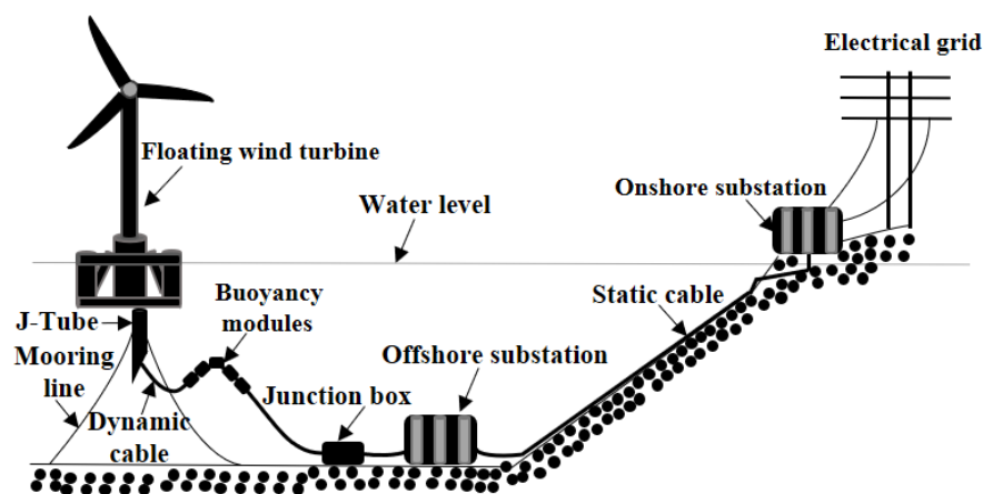
Figure 1. Power transmission system of floating offshore wind turbine.
