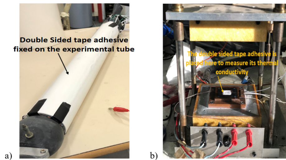
Figure 8. Double adhesive tape on (a) experimental tube (b) hot guarded plate.
