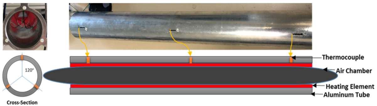
Figure 3. Schematic for the experimental tube.
