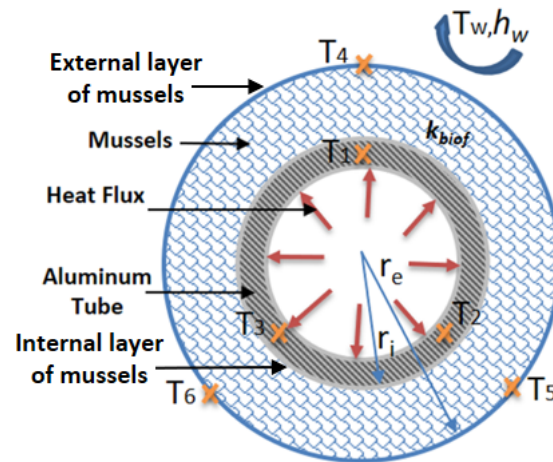
Figure 7. Middle cross-section of the aluminum tube with uniform mussels colonization.
