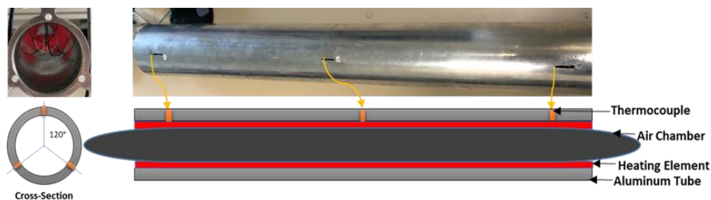
Figure 3. Schematic for the experimental tube.
