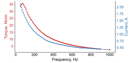
Fig. 7. Measured torque and current per phase as a function of frequency.
