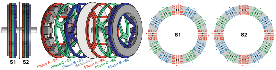
Fig. 4. The winding design of the Axial-DSIM (The three-layer planar, double-layer winding design).
