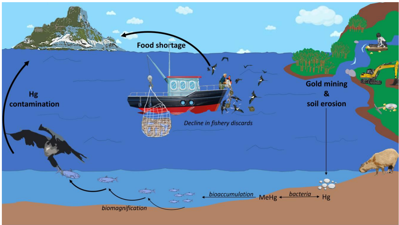
Figure 1. Graphic representation of the stress factors from French Guiana. Hg from gold mining and soil erosion is converted into MeHg, which bioaccumulates and biomagnifies within food webs. Adult frigatebird exposed to high Hg contamination may suffer its toxic effects at the physiological level (e.g. reduced parental care). Furthermore, frigatebirds are likely facing food shortage due to the decline in discards associated with shrimp trawlers and may struggle to provide food to their chicks.
