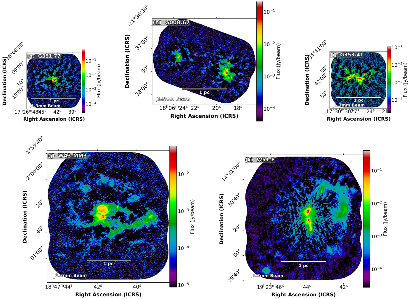
Fig. 2. (Continued) 1.3 mm continuum ALMA 12 m array images of the Intermediate clouds: G351.77 (panel g), G008.67 (panel h), G353.41 (panel i), W43-MM3 (panel j), and W51-e (panel k).
