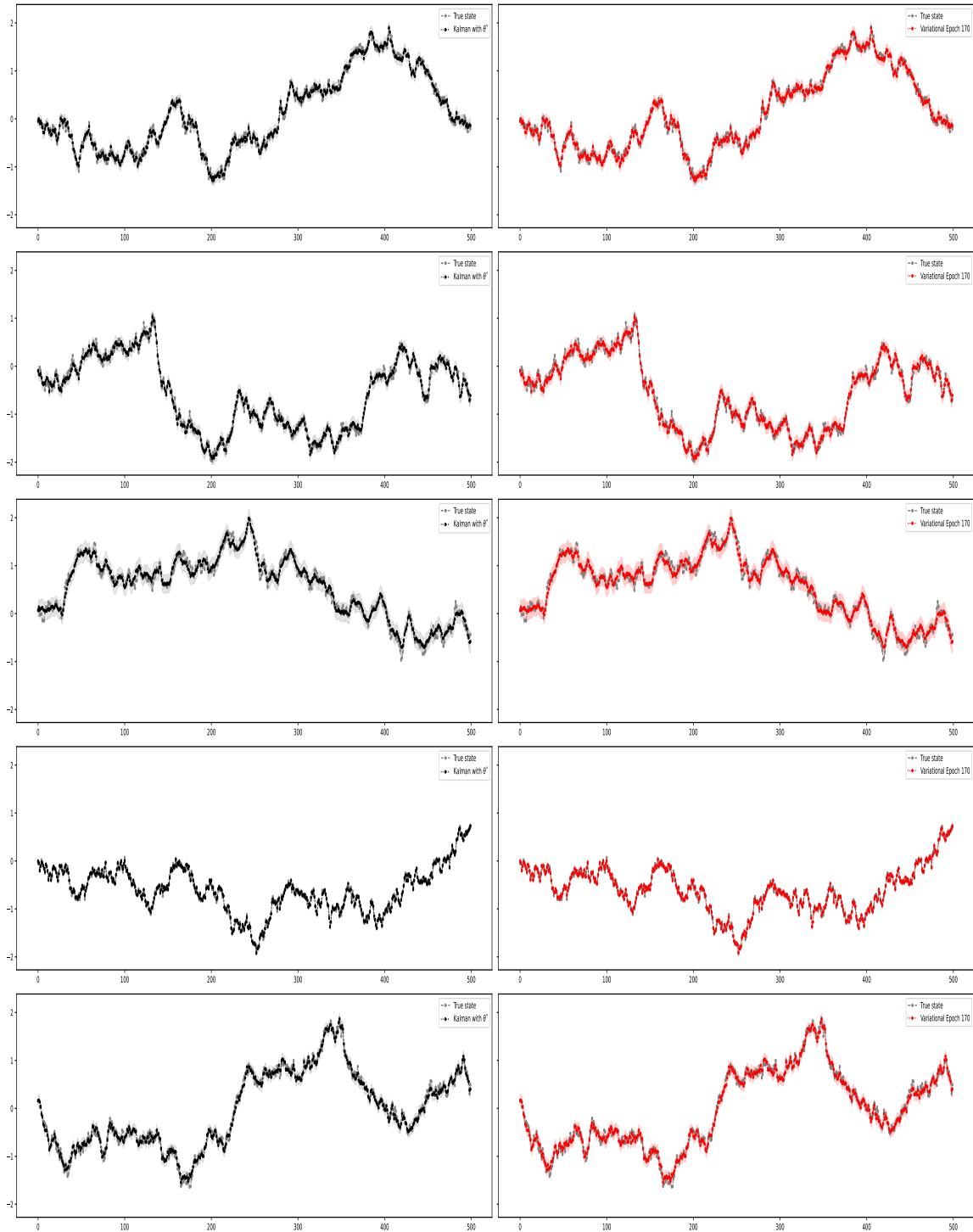
Figure 7: Example of smoothed states when the dimension of the state space is 5 and the observations is 5. Left column: component-wise (from top to bottom) smoothed states with true parameters \theta . Right column: same thing with learnt parameters \lambda . The dashed fillings are the 95% confidence intervals. The horizontal axis is the time axis.
