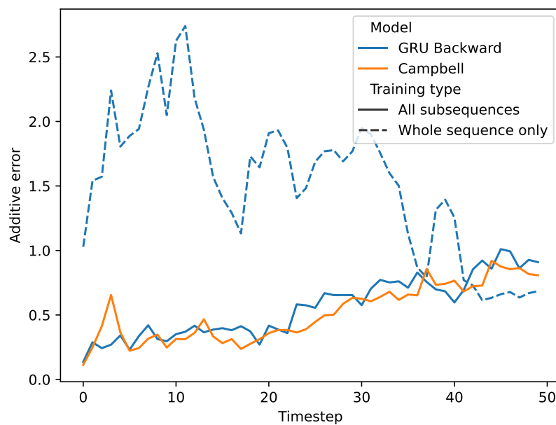
Figure 5: |q_{0:n}^\lambda h_{0:n} - \phi_{0:n}^\theta h_{0:n}| for \tilde{h}_k(x_k, x_{k+1}) = x_k when training the GRU Backward model in two different ways, alongside the solution of Campbell et al. (2021)
