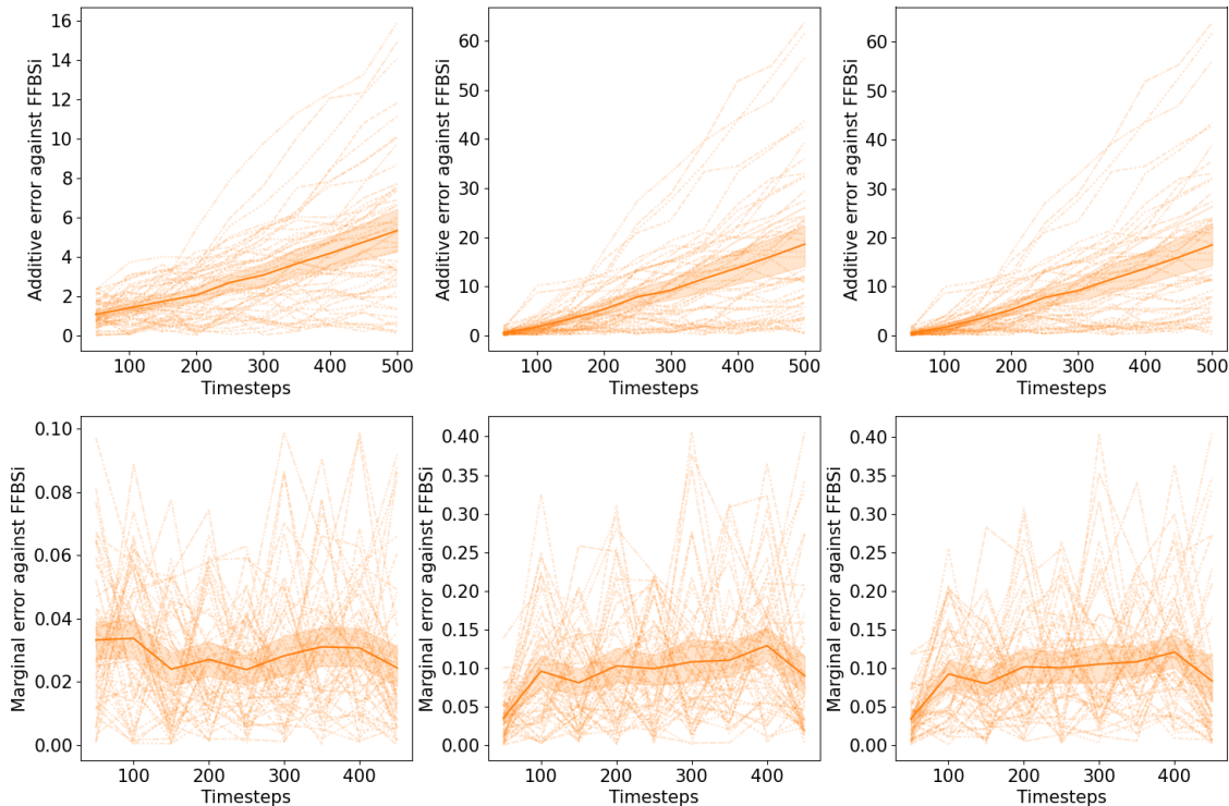
Figure 3: Additive (top) and marginal (bottom) errors against FFBSi estimates on the chaotic data with the Conjugate Backward model on three types of functionals, from left to right: (i) \tilde{h}_k(x_{k-1}, x_k) = \|x_k\|_1 (ii) \tilde{h}_k(x_{k-1}, x_k) = x_k^T x_k (iii) \tilde{h}_k(x_{k-1}, x_k) = x_{k-1}^T x_k .
