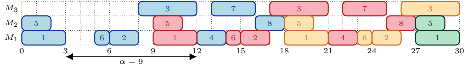
Figure 2: A periodic schedule associated with the CJSP instance with WIP = 2 .
