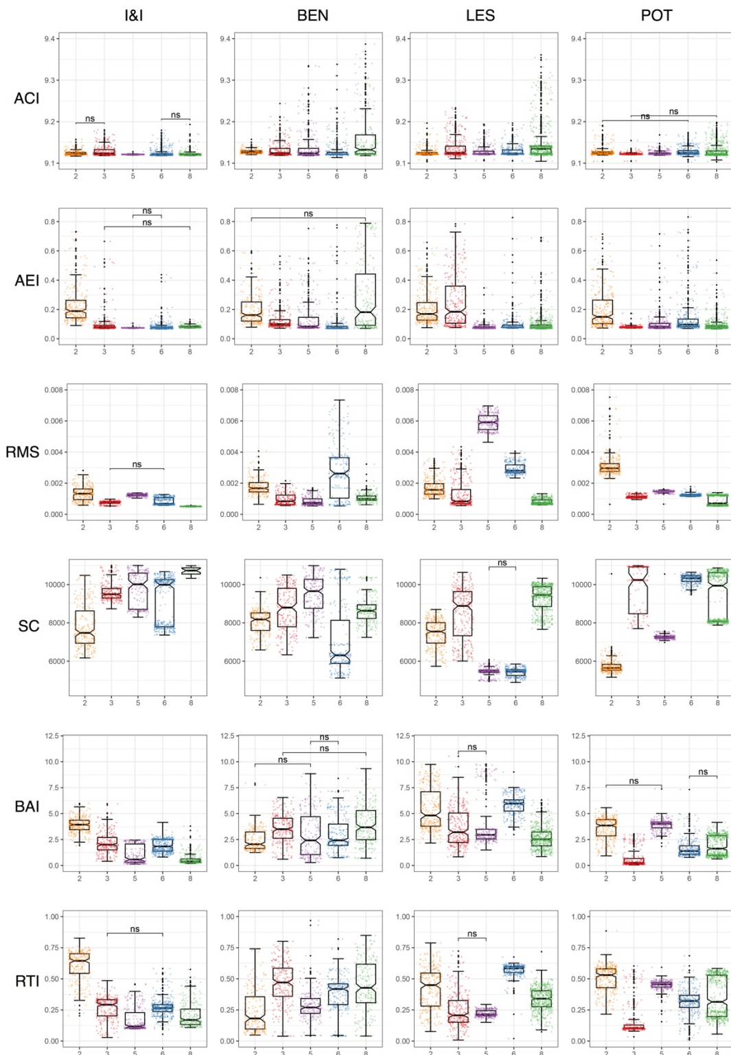
Fig 3 Tukey's box and whisker plots for AIs values (rows) across days for each WC for each study site (columns). Horizontal lines represent medians; the box represents the interquartile range; whiskers represent min and max values within 1.5 IQR. Non-significant differences ( p < 0.05 ) between sites are denoted by bars ns. Individual AI values shown as points.
