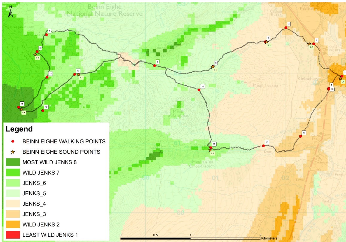
Figure 1. Example of transect walk along gradient of Jenks wildness classes for Scottish site Beinn Eighe National Nature Reserve (BEN) on the Scottish west coast (Lat 57° 36' 8.6004" N, Long -5° 19' 0.624" W) showing human perception and acoustic survey points. See Supplementary Material A for corresponding maps of other sites.
