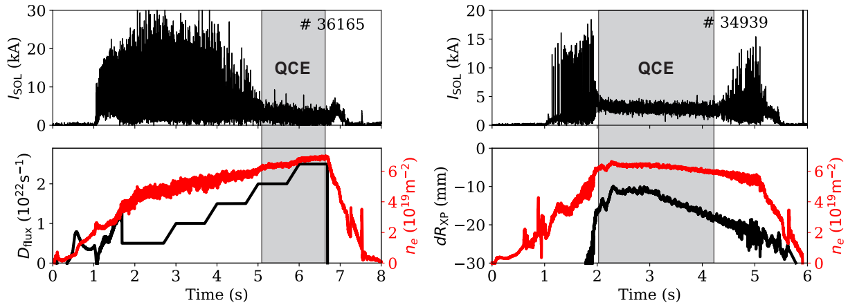
FIG. 5: The QCE regime appears when type-I ELMs, detected in the divertor current I_{\text{SOL}} , vanish at high density (left) and in configurations close to double null (right), measured by the distance of the separatrix from the second X-point, dR_{\text{XP}} .
