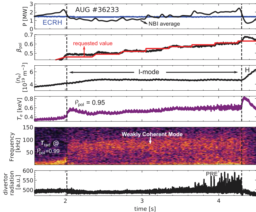
FIG. 4: Time traces of I-mode discharge parameters, where the plasma \beta_{pol} was feedback controlled via the NBI power. The weakly coherent mode appears in the spectrogram of the ECE radiation measured with a channel close to the separatrix. Close to the I-H transition, pedestal relaxation events (PRE) are visible in the divertor radiation signal (adapted from Ref. [46]).
