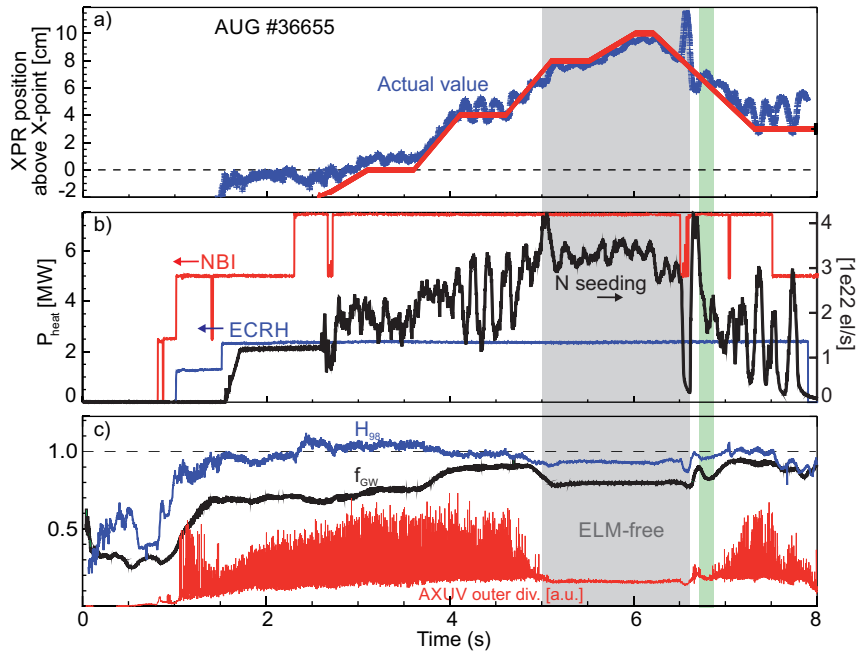
FIG. 8: XPR position control (a) by nitrogen seeding (b) with an ELM-free phase at high confinement and density (c) (adapted from Ref. [3]).
