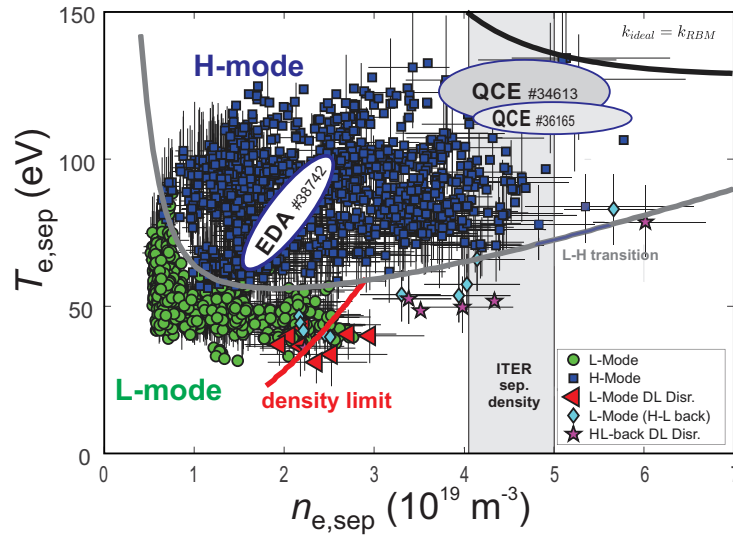
FIG. 7: Operational boundaries in the separatrix electron plasma parameter space. Symbols mark L- and H-mode data ( \circ and \square ), disruptive discharges in L-mode or after back transition to L-mode are marked as \triangleleft and \star , respectively. \diamond symbols mark L-mode phases following an H-L back transition prior to an L-mode disruption. (adapted from Ref. [75]). The parameter ranges of an EDA H-mode and two QCE discharges are overlaid and the separatrix density range expected for ITER [79,80] is indicated.
