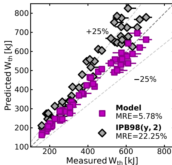
FIG. 1: Comparison of the thermal energy content in AUG H-mode plasmas as derived from the IMEP model and from the IPB98(y,2) scaling with experimental values (adapted from Ref. [6]).
