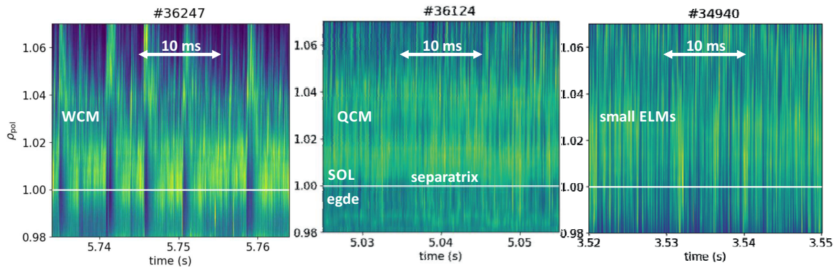
FIG. 6: Density fluctuations measured with the helium beam diagnostics across the separatrix during (from left to right) I-mode, EDA H-mode and QCE discharges phases (adapted from Ref. [73]).
