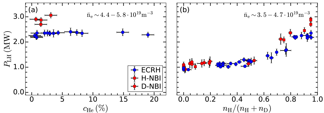
FIG. 3: Dependence of the L-H power threshold values in hydrogen discharges as function of the helium content (a) and for a transition from a pure deuterium to a hydrogen plasma (b). Symbols indicate different heating beams (H or D NBI) and ECRH plasmas (adapted from Ref. [34] with additional data [35]).
