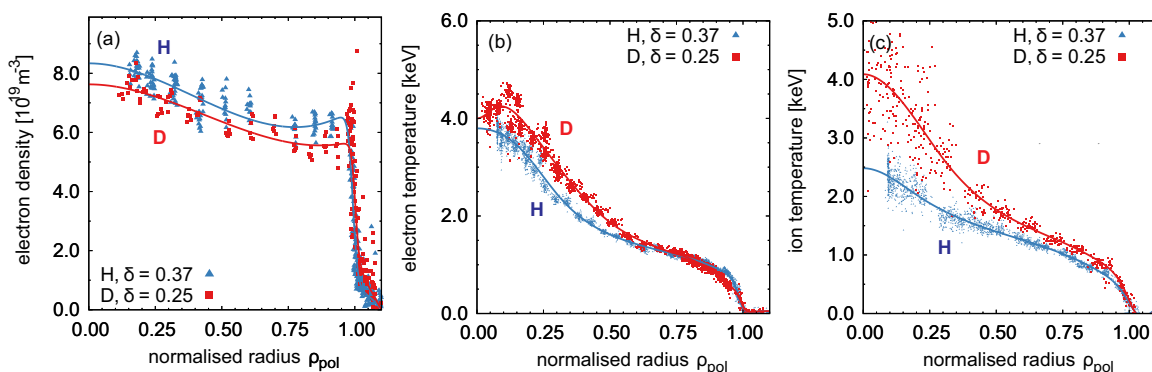
FIG. 2: Kinetic profiles of a pair of hydrogen and deuterium H-mode plasmas, where the edge profiles were matched while the source profiles are kept similar (adapted from Ref. [12]).
