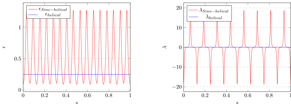
Figure 3: The dimensionless parameters \varepsilon , (a), and \lambda , (b), for the sine-helical and the helical geometries. To compare them, the parameters are rescaled as function of s = 2\pi M/\hat{\theta} \in [0, 1] , where M = M_{\text{sh}} = 2 for the sine-helical channel.
