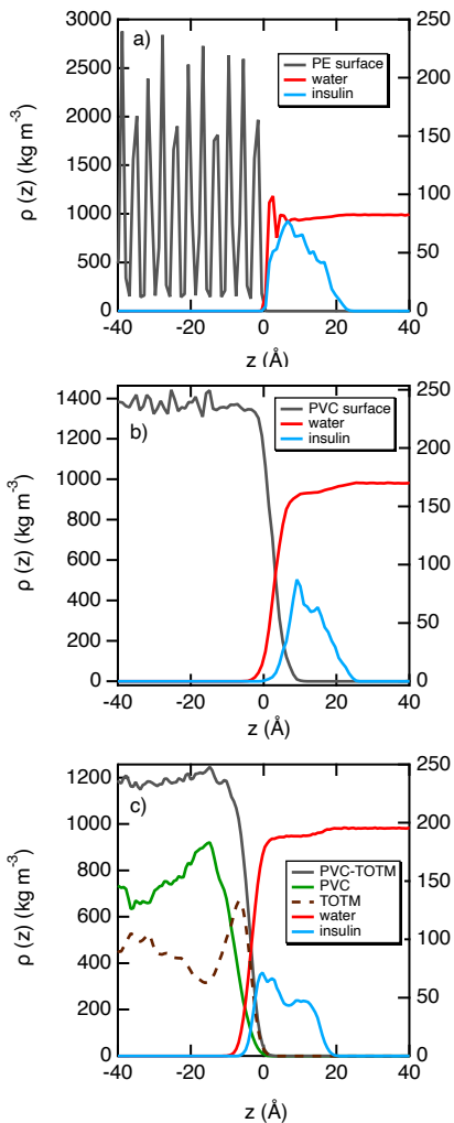
Figure 8: Atomic density profiles of PVC, TOTM, insulin and water molecules calculated in the direction perpendicular to the surface where z represent the position of atoms. The density profiles of insulin should be read on the right-hand scale. The profiles of a), b) and c) represent the adsorption of insulin onto the PE, PVC and PVC-TOTM materials, respectively.
