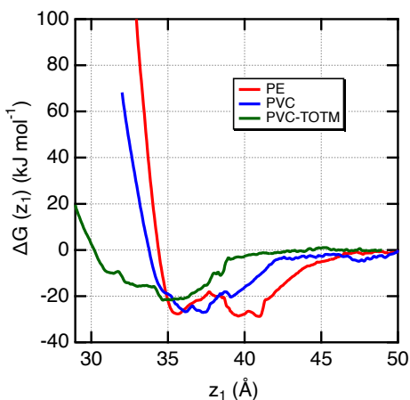
Figure 4: Gibbs free energy profiles \Delta G(z_1) of the adsorption process of insulin onto polymeric materials (PE, PVC and PVC-TOTM) as a function of the z_1 -separation distance between the centers-of-mass.
