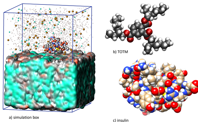
Figure 2: a) Typical configuration of one aspart insulin molecule in interaction with a plasticized PVC including solvent molecules and counter-ions. b) and c) show the chemical structures of the TOTM and insulin molecules.
