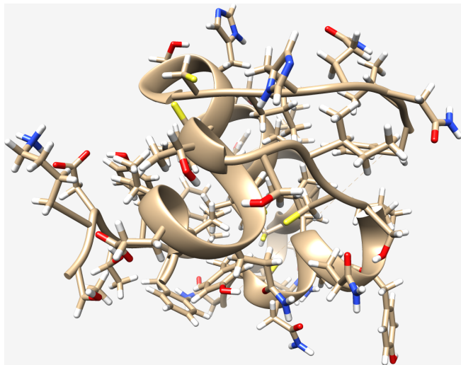
Figure 1: Monomer aspart insulin formed by two peptide chains A and B. Chain A is made up of 21 amino acid residues leading to two \alpha -helices. Chain B contains a central \alpha -helice formed by 30 residues. The two peptide chains are linked by two inter-chains A7(Cys)-B7(Cys) and A20(Cys)-B19(Cys) disulphide bridges (yellow). Another disulphide bridge occurs in the A-chain between A6(Cys)-A11(Cys).
