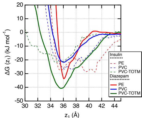
Figure 6: Gibbs free energy profiles \Delta G(z_1) calculated during the adsorption process of insulin and diazepam molecules onto PE, PVC and PVC-TOTM surfaces as a function of the z -separation distance between the centers-of-mass defined here by z_1
