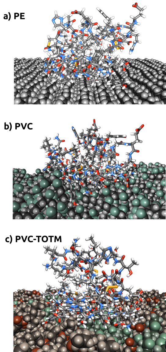
Figure 5: Typical configurations representative of the region of minimum Gibbs free energy for the a) PE, b) PVC and c) PVC-TOTM materials. The water molecules have been omitted for clarity.
