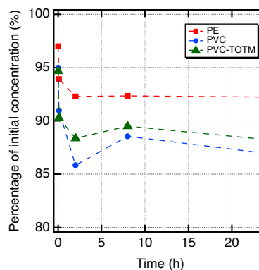
Figure 3: Experimental evolution of insulin concentration in static contact with PE and PVC tubings compared to initial concentrations. The error-bars, less than 1%, cannot be read with the scale used.
