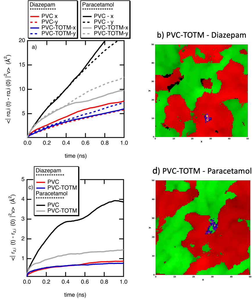
Figure 7: (a) x and y and (c) z components of mean square displacements versus time of adsorbed drug molecules on pure PVC and PVC-TOTM surfaces. (b) and (d) positions of diazepam and paracetamol molecules along the x and y directions. The blue color represents the positions of the drug, red the positions of the plasticizers and green the PVC molecules.
