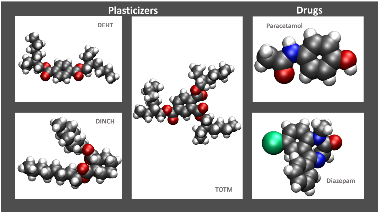
Figure 1: Conformations of the plasticizers (DEHT, DINCH and TOTM) and drugs (paracetamol and diazepam). The hydrogen, carbon, oxygen, nitrogen and chlorine atoms are represented in white, grey, red, blue and green, respectively.
