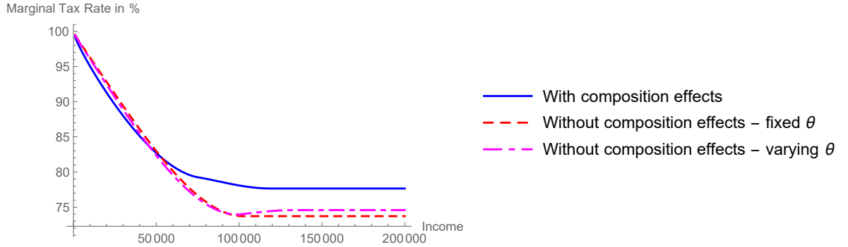
FIGURE 1. Optimal marginal tax rates with composition effects (solid blue line), without composition effects and fixed \theta (dashed red lines), without composition effects and varying \theta (dash-dotted pink lines)
