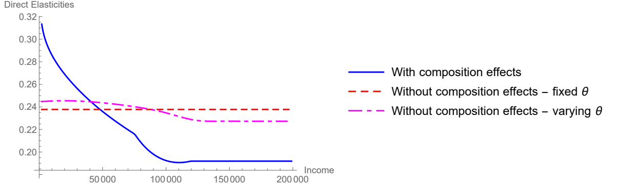
FIGURE 4. Mean direct elasticities with composition effects (solid blue line), without composition effects and fixed \theta (dashed red lines), without composition effects and varying \theta (dash-dotted pink lines)
