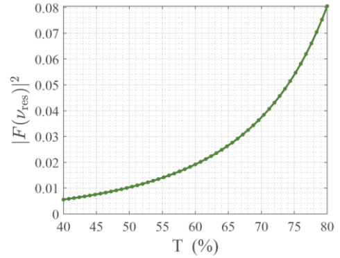
Fig. 3: Intensity transfer function of the cavity probed in transmission at resonance frequency \nu_{\text{res}} versus T the intracavity transmission
