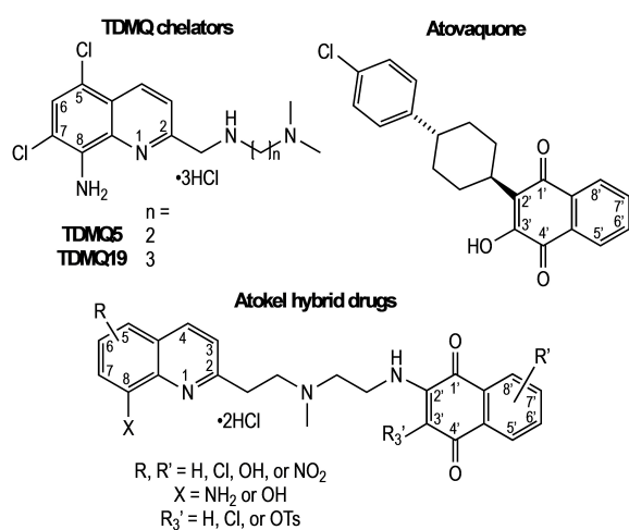
Figure 1. Structures of TDMQ chelators, atovaquone, and the Atokel hybrid drugs.
