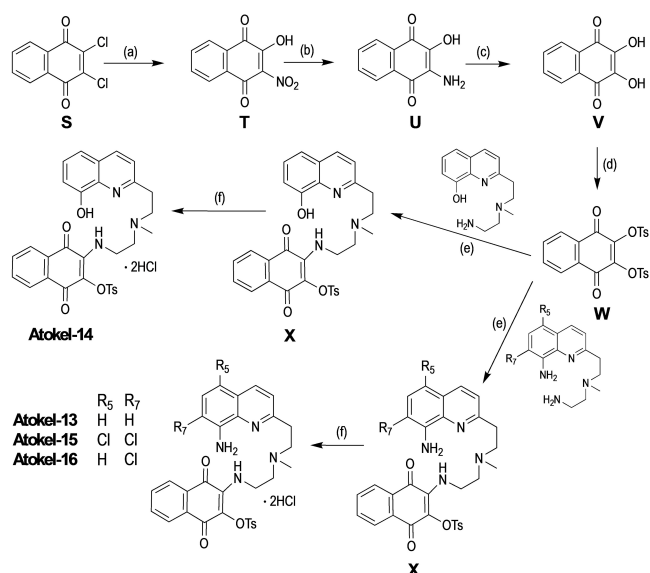
Scheme 4. General scheme of the syntheses of Atokel-13-16 : (a) NaNO 2 , acetone/methanol (1/1, v/v), reflux, 3 h; (b) Na 2 S 2 O 4 , H 2 O, RT, 2 h; (c) H 2 SO 4 (30%), reflux; (d) TsCl, Et 3 N, THF, RT, 24 h; (e) in presence of compound G (Scheme 1) or P (Scheme 3), K 2 CO 3 , CH 3 CN, RT, overnight; (f) HCl, EtOH, CH 2 Cl 2 .
