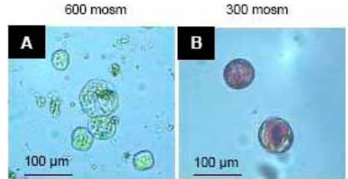
Fig. 5 - Protoplasts derived from six-day-old Cakile maritima cell suspension maintained in 0.6 M sorbitol (A) or 0.3 M sorbitol (B).
