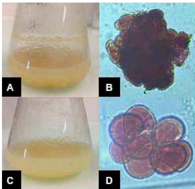
Fig. 2 - Establishment of Cakile maritima cell suspensions. (A) Dense suspension cells grown in flask after two months feeding and (B) corresponding cell aggregates magnified 300X. (C) Dense suspension cells grown in flask after 1.5 months of subculture after feeding and (D) corresponding cell aggregates magnified 300X.
