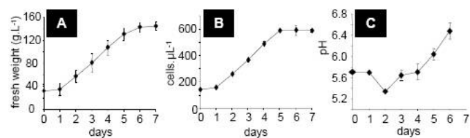
Fig. 3 - Growth pattern of Cakile maritima cell suspension determined by fresh weight (A) or cell density measurements (B). Evolution of the medium pH during cell suspension growth. Bars indicate mean \pm SD of at least three experiments.
