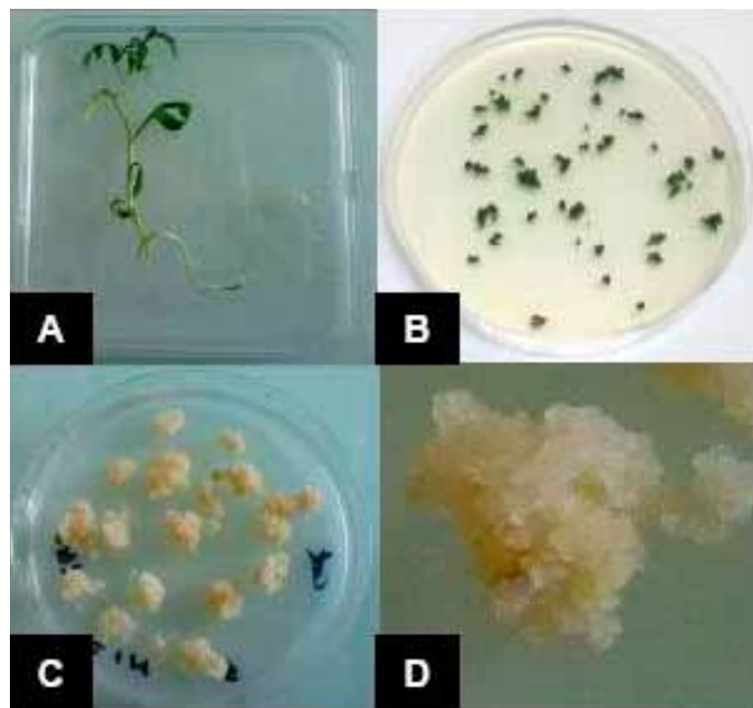
Fig. 1 - Establishment of Cakile maritima calluses. (A) Three-week-old C. maritima seedling grown from sterilized seed. (B) Slices of leaf and rod were finely cut for callus generation. (C) One-month-old calluses derived from rod and leaf slices. (D) Magnification of a callus.
