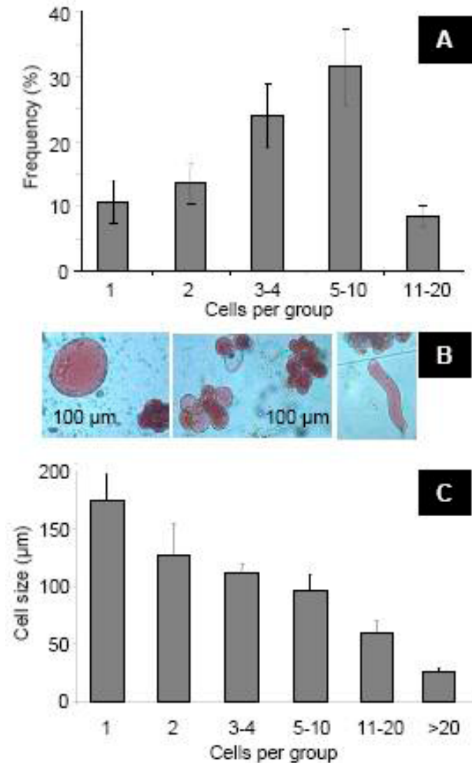
Fig. 4 Morphology of six-day-old Cakile maritima suspension cells. (A) Frequency of cell groups in the culture. (B) Different morphologies of cells. (C) Sizes of the cells according to the size of the cell groups. At least 250 cells were analyzed; bars indicate mean \pm SD.
