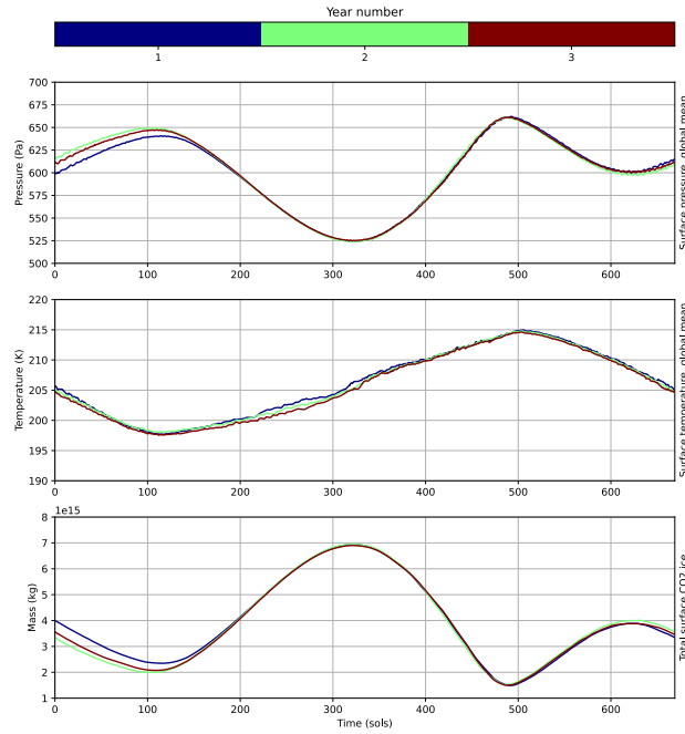
Figure 23: Same as 21, but for MPCO2+H2OCN simulation.
