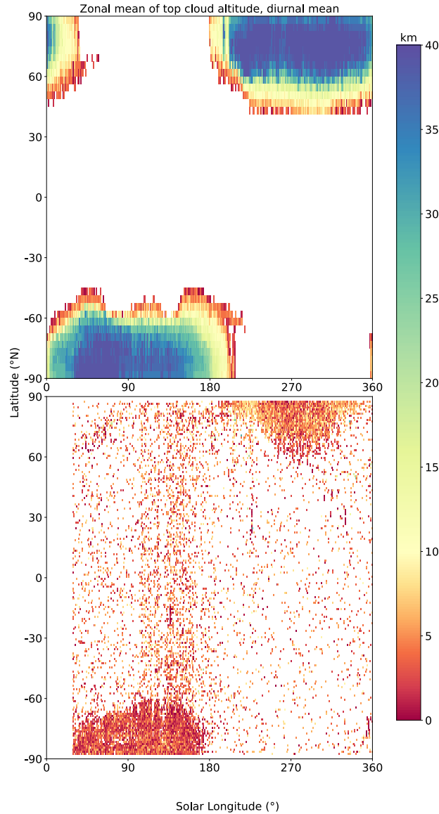
Figure 4: Zonal mean of CO 2 ice cloud top altitudes in the polar regions. Top: Cloud tops in MPCO 2 +H 2 OCN simulation as should be seen by MOLA when applying the approach of Pettengill and Ford (2000); bottom: Cloud top altitudes from MOLA observations (Neumann et al., 2003) averaged in a 1° × 1° grid.
