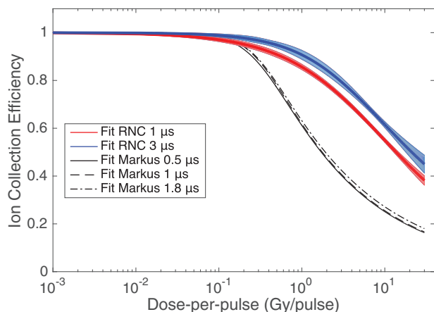
FIGURE 5 Ion collection efficiency of the RNC as a function of the dose per pulse, for pulse lengths of 1 \mu\text{s} (red curve) and 3 \mu\text{s} (blue curve), fitted with the logistic recombination model. The uncertainties on ICE (see section 2.5) are represented by the shaded region around the main curves. The RNC ICE results are compared with those of the Markus Advanced ion chamber of PTW for pulse lengths of 0.5–1.8 \mu\text{s} , as published by Petersson et al. 32
