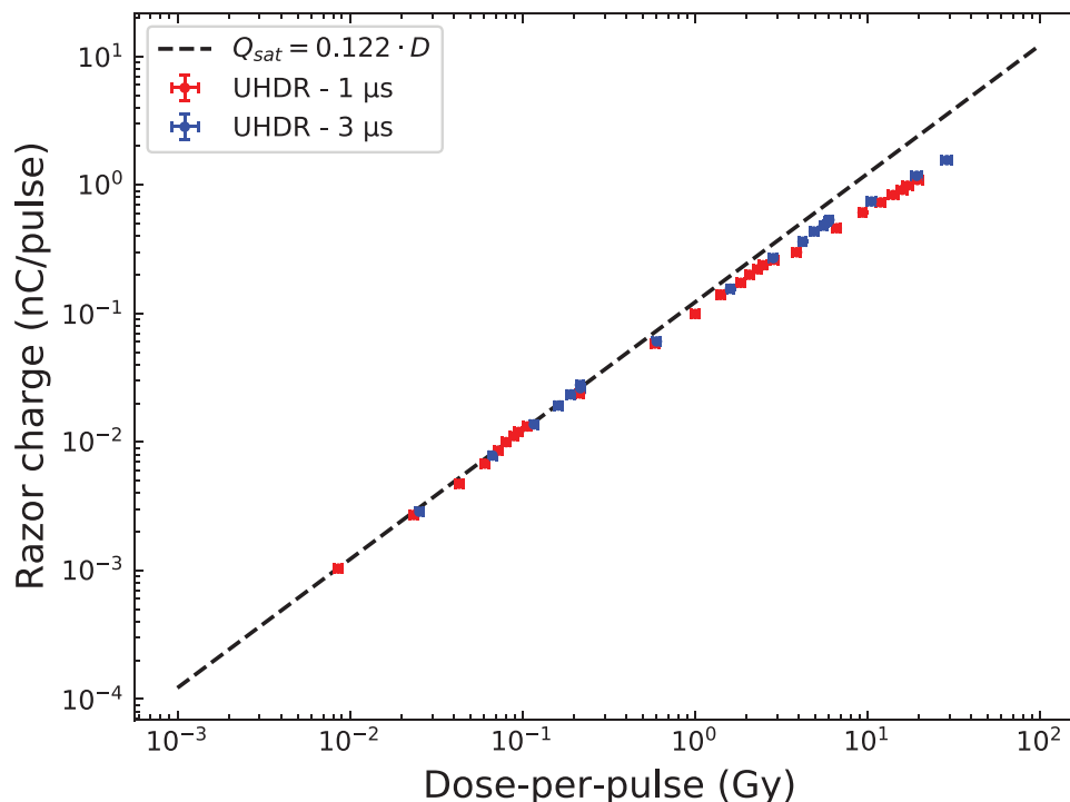
FIGURE 4 RNC charge response as a function of the dose-per-pulse (DPP). Two series were performed at pulse lengths of 1\ \mu\text{s} (red dots) and 3\ \mu\text{s} (blue dots), with DPP ranging from 0.01 to 30 Gy. The black linear dashed curve represents the saturation charge Q_{\text{sat}} , that is, the charge that would be collected to the RNC electrodes if no recombination occurred. The uncertainty on DPP was of 5% (horizontal error bars) and that on the RNC charge response was of 0.43% (vertical error bars)
