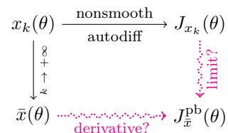
Figure 1: We study existence and meaning of J_{\bar{x}}^{\text{pb}} as a derivative of \bar{x} , compatible with automatic differentiation of the iterates (x_k(\theta))_{k \in \mathbb{N}} .
