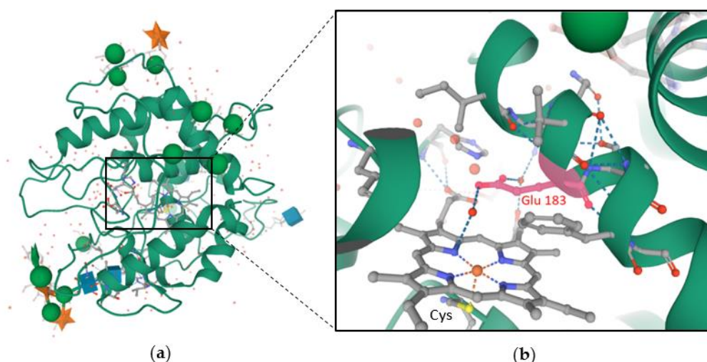
Figure 4. (a) Crystal structure of heme-chloroperoxidase from Leptoxiphium fumago (PDB ID: 1CPO). (b) Active site with glutamic acid 183 colored in pink.
