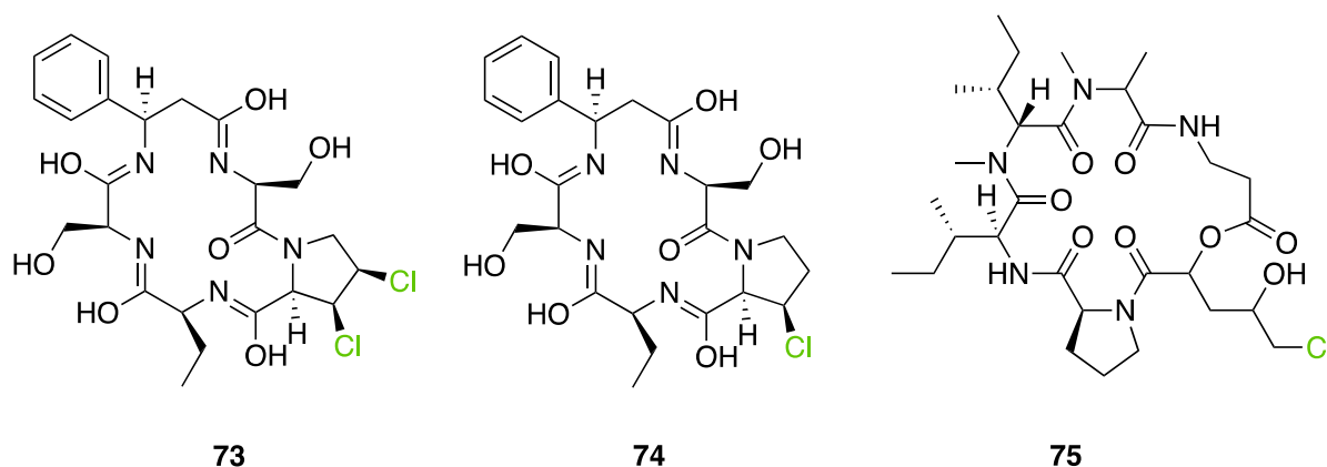
Figure 31. Example of halogenated non ribosomal peptides found in this specific cluster 7, cyclochlorotine (73) and cyclochlorotine B (74) from Penicillium islandicum , destruxin-A4-cyclohydrin (75) from unknown fungi.
