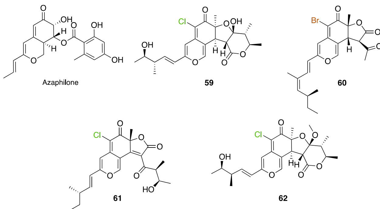
Figure 27. Representative azaphilone-type metabolites from cluster 3: 11-epichaetomugilin A (59) from Chaetomium sp.; 5-bromoochrephilone (60) from Penicillium sp.; chaetoviridin E (61) and chaetomugilin B (62) from Chaetomium sp.
