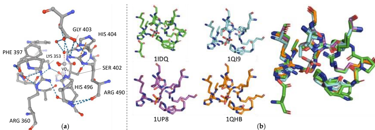
Figure 7. (a) Vanadate ( \text{VO}_4^{3-} )-binding pocket in vCPO from Curvularia inaequalis (PDB ID: 1IDQ). (b) Structural overlay of active sites from different vHPOs crystallized: vCPO from C. inaequalis (PDB ID: 1IDQ), vHPO from A. nodosum (PDB ID: 1QI9), vBPO from C. pilulifera (PDB ID: 1UP8), and vBPO from C. officinalis (PDB ID: 1QHB).
