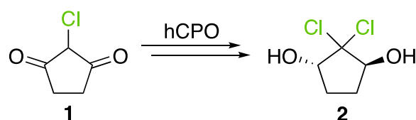
Figure 6. 2-chlorocyclopentane-1,3-dione (1) chlorination to form caldariomycin (2) inspired by [84].
