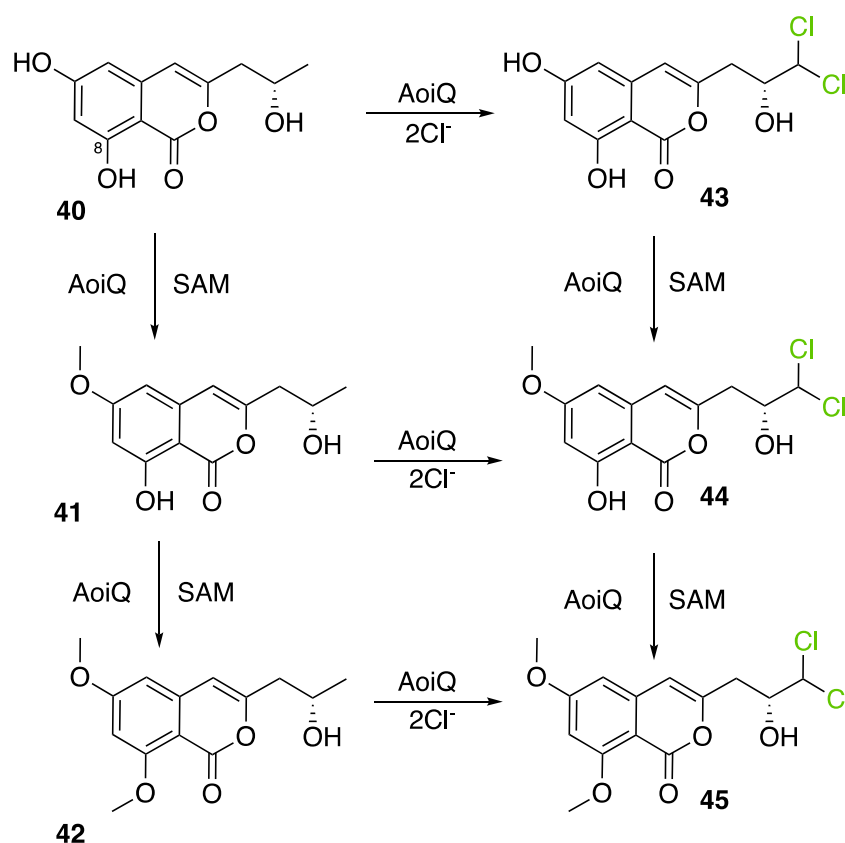
Figure 21. Biosynthetic route examples of the hybrid enzyme AoiQ described in Aspergillus oryzae on diaporthin derivatives de- O -methyl diaporthin (40), diaporthin (41), 8-methoxy diaporthin (42), de- O -methyl-dichloro diaporthin (43), dichloro diaporthin (44), and 8-methoxy-dichloro diaporthin (45).
