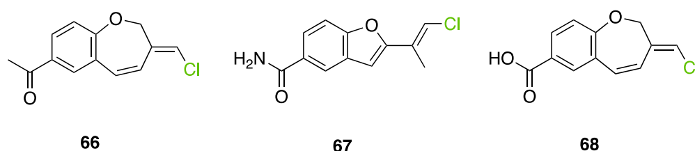
Figure 29. Some metabolites from cluster 5: pterulone ( 66 ), calocerin ( 67 ), and 2,3-dihydro-1-benzoxepin derivative 4a ( 68 ).
