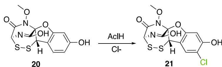
Figure 17. Chlorination of dechloroaspirochlorine (20) by AclH in A. oryzae to form aspirochlorine (21).
