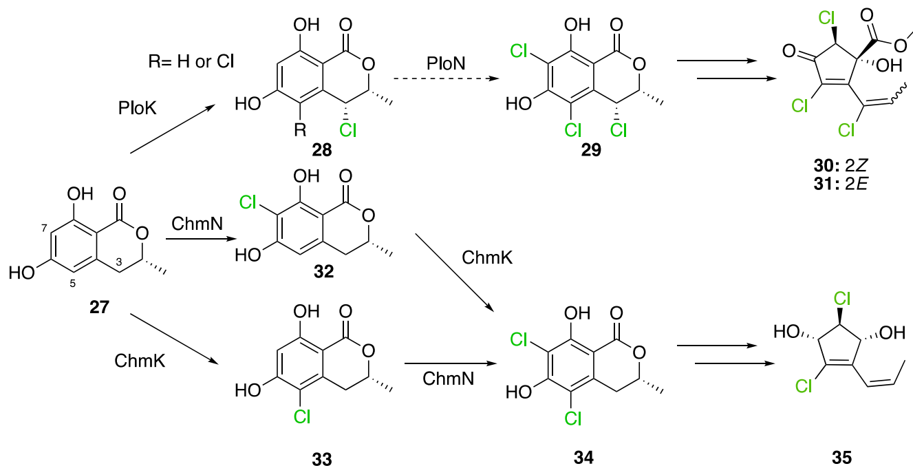
Figure 19. Halogenation of ( R )-6-hydroxymellein (27) by PloK and PloN in L. palmae , and in H. velutinum by ChmK and ChmN. If R = H, (2 R ,3 R )-3-Chloro-6-hydroxymellein, if R = Cl, (2 R ,3 R )-3,5-Dichloro-6-hydroxymellein (28). (2 R ,3 R )-3,5,7-Trichloro-6-hydroxymellein (29), palmaenone A (30), palmaenone B (31). ( R )-7-Chloro-6-hydroxymellein (32), ( R )-5-chloro-6-hydroxymellein (33), ( R )-5,7-dichloro-6-hydroxymellein (34), and cyclohelminthol IV (35).
