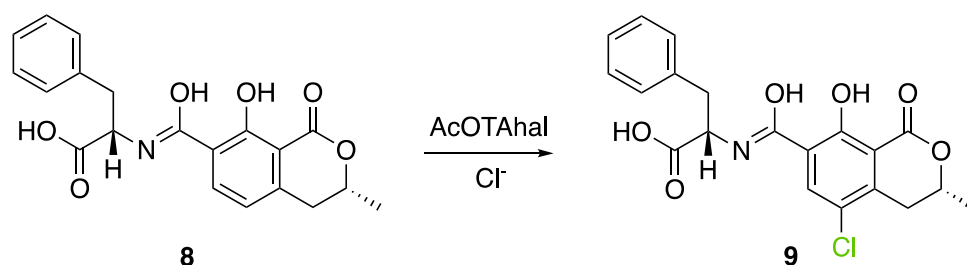
Figure 13. The FDH AcOTAhal catalyzes the chlorination of ochratoxin B (8) to form ochratoxin A (9) in Aspergillus carbonarius [33].
