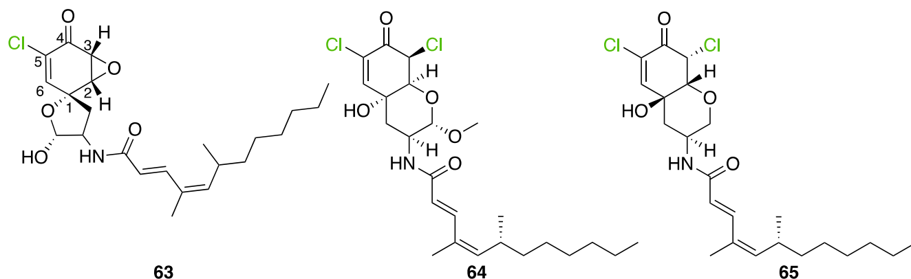
Figure 28. Metabolites present in cluster 4, aranochlor A ( 63 ) from Pseudoarachniotus sp., dankastatin A ( 64 ) and B ( 65 ) from Gymnascella sp.
