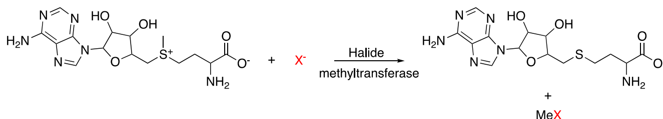
Figure 23. Example of a halide methyltransferase catalyzed reaction.
