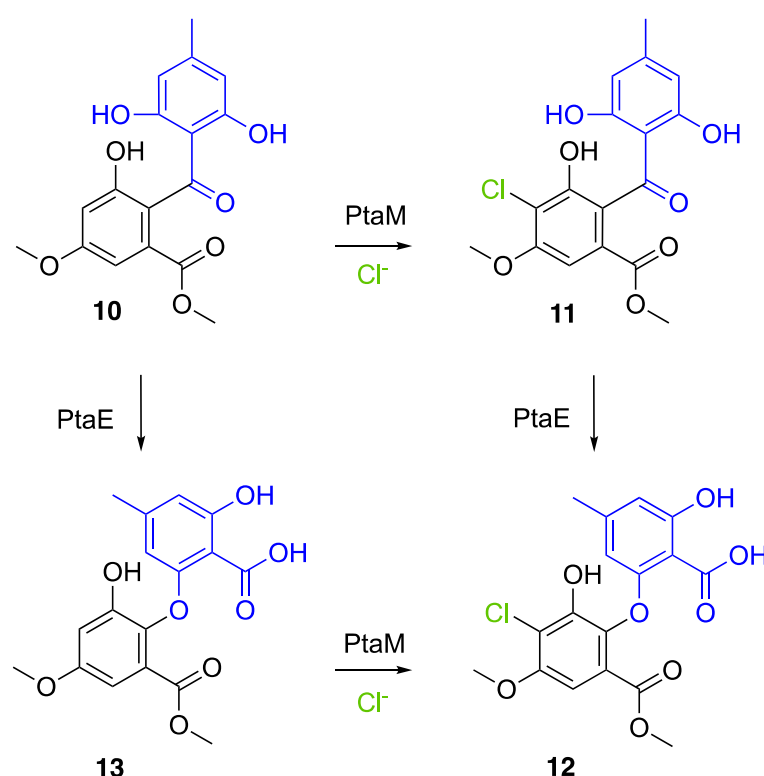
Figure 14. Chlorination of isosulochrin ( 10 ) by PtaM in P. fici to obtain chloroisosulochrin ( 11 ), a precursor of pestheic acid ( 12 ). Isosulochrin ( 10 ) can be oxidized by PtaE to form RES-1214-1 ( 13 ), which is chlorinated by PtaM to form pestheic acid ( 12 ) in Pestalotiopsis sp.
