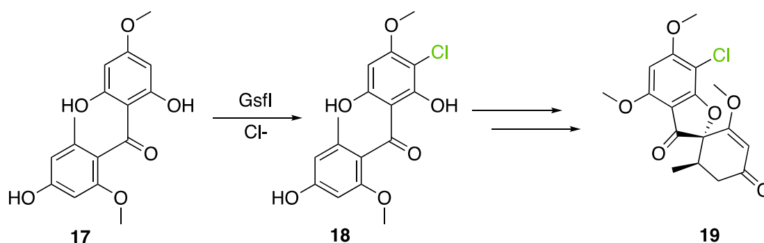
Figure 16. Chlorination of griseophenone C (17) by GsfI to form griseophenone B (18), precursor of griseofulvin (19) in P. aethiopicum .
