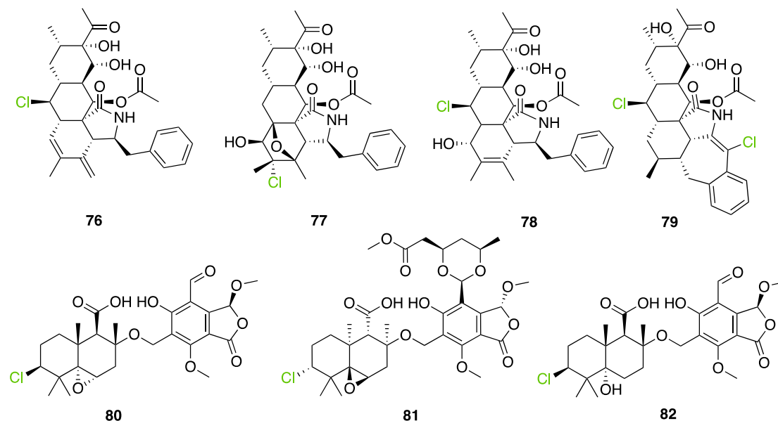
Figure 32. Compounds belonging to cluster 8: curtachalasin derivatives L ( 76 ), I ( 77 ), and K ( 78 ) and xylarichalasin A ( 79 ); and cluster 9: pestalotiopens A ( 80 ), B ( 81 ), and C ( 82 ).
