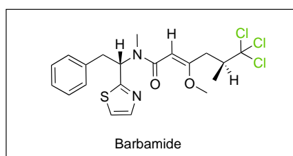
Bacterial compound
