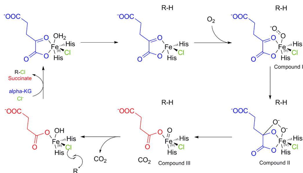
Figure 22. Catalytic cycle of NHFe halogenase inspired by Butler et al. [75].
