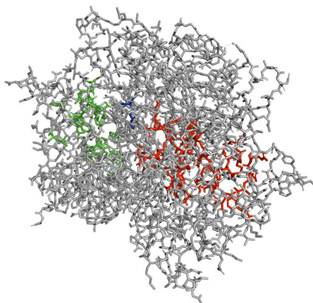
Figure 9. 5WGR-crystal structure of wild-type MalA', premalbrancheamide complex: separation between substrate binding pocket (green), FAD binding pocket (red), and lysine 108 (blue) [30].
