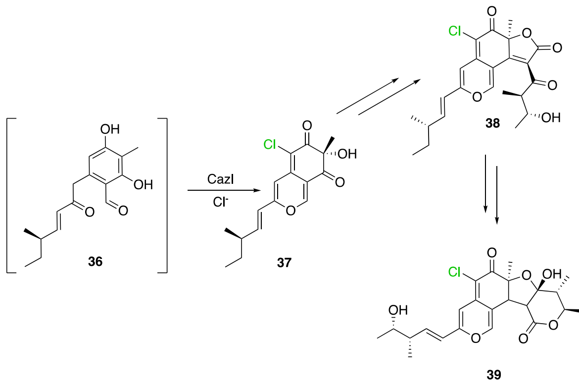
Figure 20. Chlorination of the biosynthetic intermediate (36) to obtain cazisochromen (37) in the biosynthetic pathway of chaetoviridin A (38) and chaetomugilin A (39).
