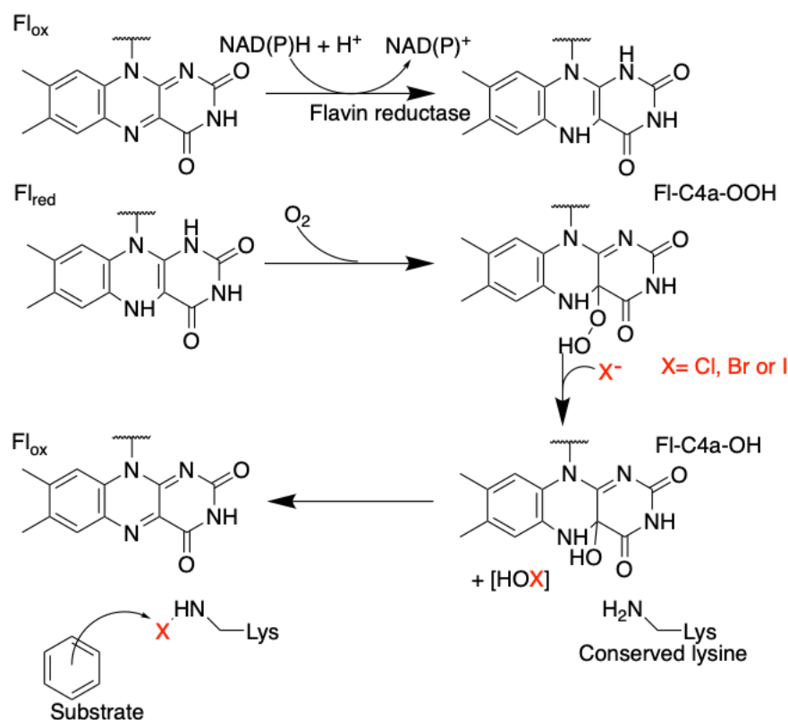
Figure 10. FDH schematic reaction mechanism inspired by [88].
