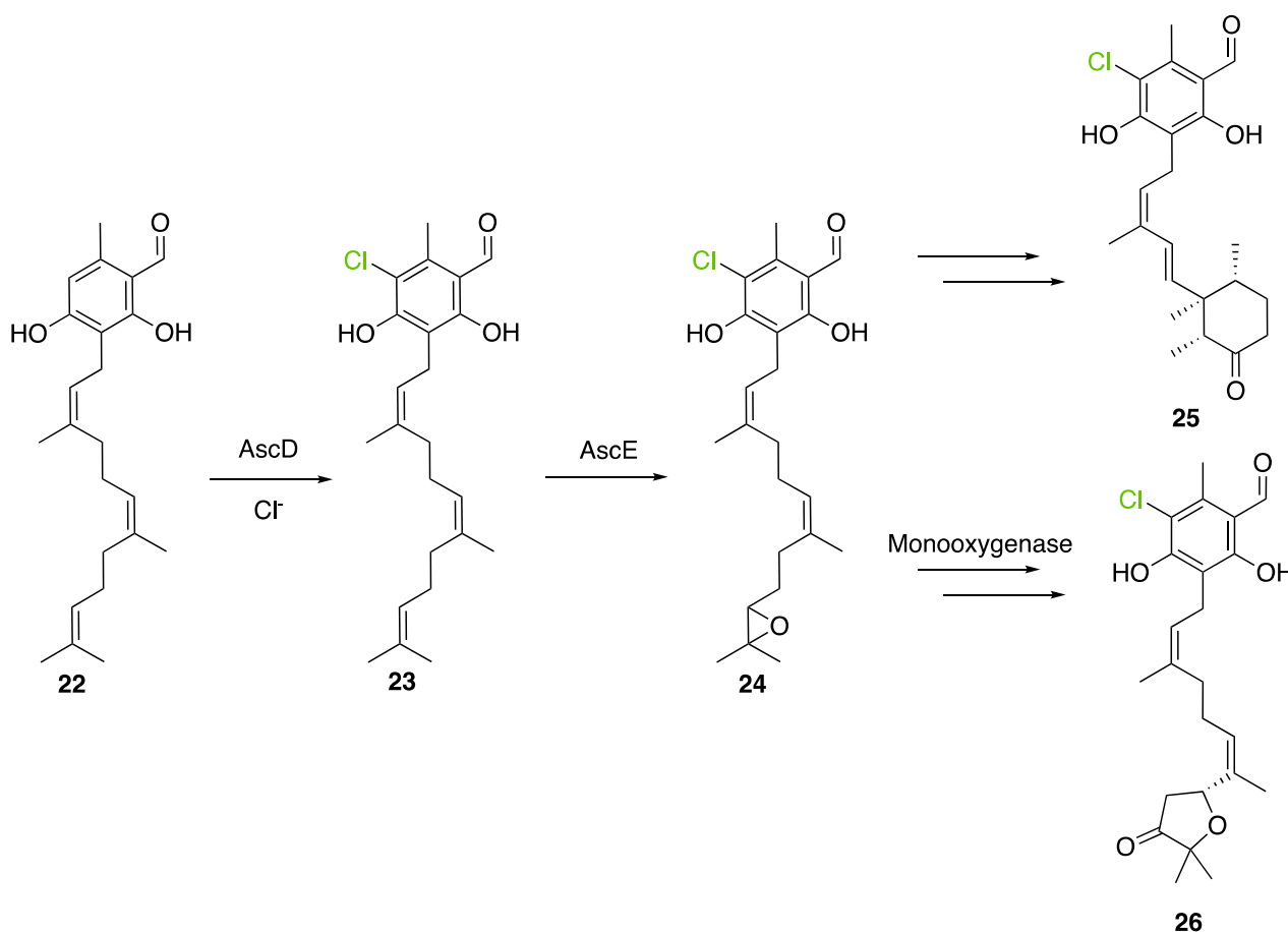
Figure 18. Chlorination of ilicicolin B (22) by AscD in A. egyptiacum to form ilicicolin A (23) and then the epoxide form (24) in the biosynthesis of ascoclhorin (25) and ascofuranone (26).
