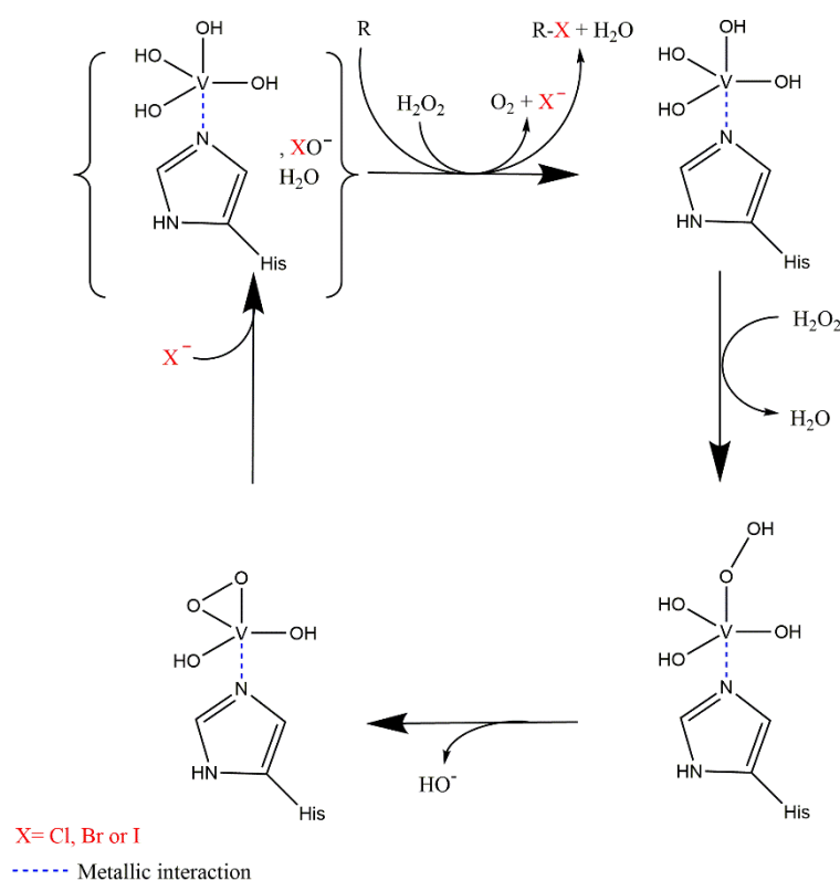
Figure 8. General halogenation mechanism of vanadium-dependent haloperoxidases inspired by [88].
