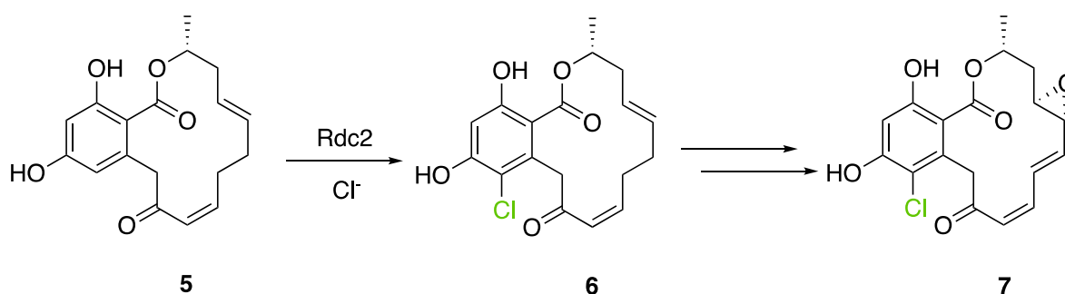
Figure 12. ( R )-Monocillin II (5) chlorination by Rdc2 to form pochonin D (6), precursor of radicicol (7).
