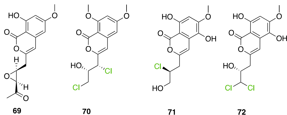
Figure 30. Metabolites displaying chlorination on aliphatic chains in the studied cluster 6, peniisocoumarin C (69) from Penicillium commune , (9R)-8-methyl-9,11-dichlorodiaporthin (70) from Hamigera fusca , and peniisocoumarin F (71) and J (72) from Penicillium commune .
