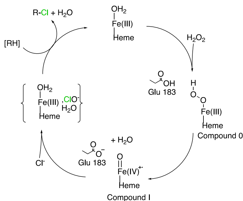
Figure 5. Schematic mechanism of hHPOs inspired by [75].
