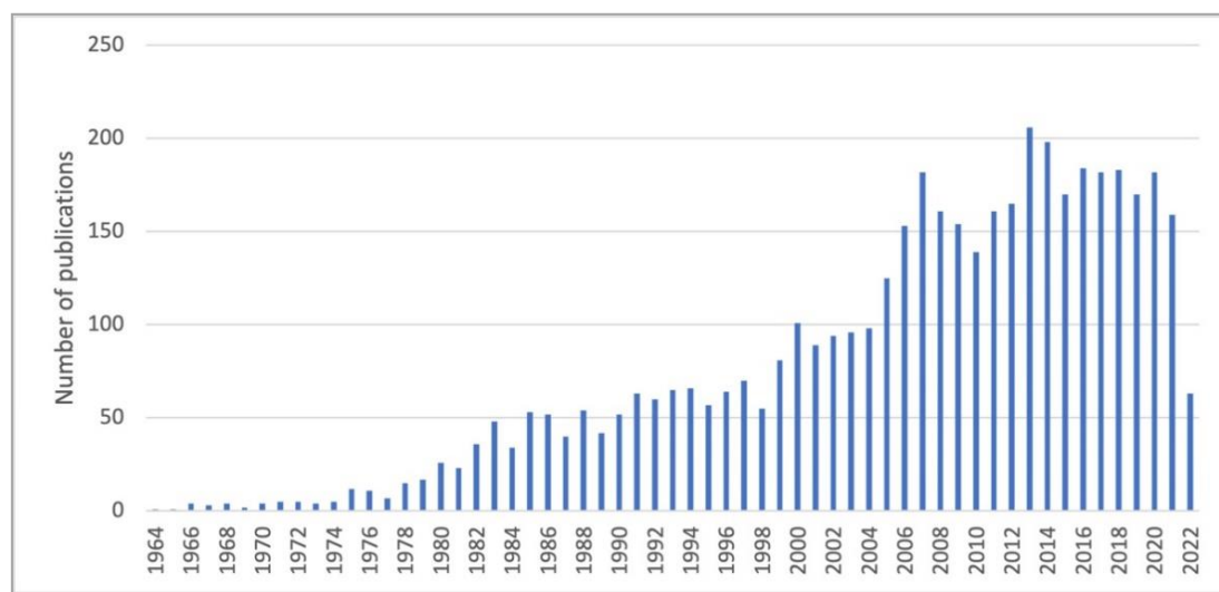
Figure 3. Evolution of the number of publications available on PubMed for halogenation enzymes (keywords used for the research on PubMed: haloperoxidase, chloroperoxidase, bromoperoxidase, iodoperoxidase, and halogenase).
