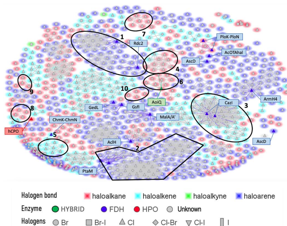
Figure 24. Similarity molecular network of the 865 halogenated fungal metabolites described in the Natural Product Atlas in 2021. This plot was created with DataWarrior software, where structures were clustered based on their similarity using the “FragFp” descriptor (set to 80% for similarity analysis). Each structure is represented by a marker whose shape is defined by the halogens present: chlorine ( \Delta ), bromine ( \circ ), iodine ( \square ), chlorine and bromine ( \diamond ), chlorine and iodine ( \nabla ), and bromine and iodine ( \square ). Structures for which a halogenating enzyme was described as being involved in their biosynthesis appeared as colored: in green for hybrid enzyme, in blue for flavin-dependent halogenases (FDH), and in red for haloperoxidases (HPO). Finally, the type of halogen bond for each molecule is represented by a halo surrounding the marker, which is blue for haloarenes, turquoise for haloalkenes, red for haloalkanes, and green for haloalkynes. Classification of the structures according to their halogen bonds was performed using the classifyR package on R Cran [147] and the Chebi descriptors. Black and numerated circles (1 to 10) correspond to studied and detailed clusters in the present review.
