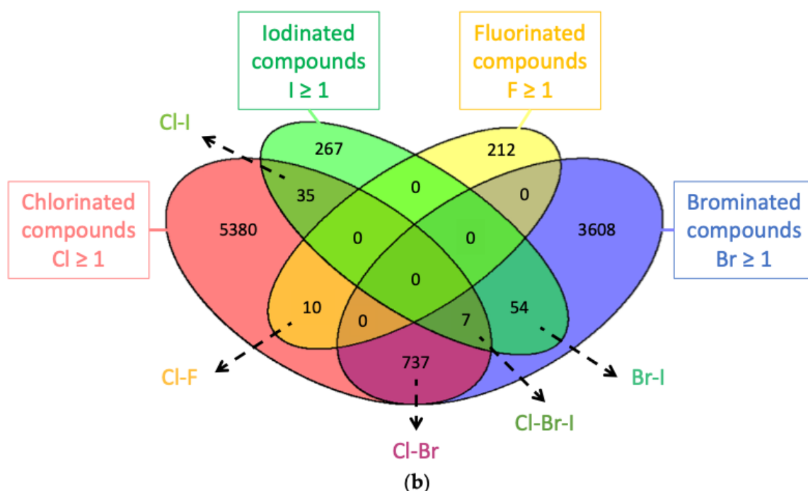
Figure 1. (a) Distribution of all halogenated natural products recorded in the Dictionary of Natural Products in March 2021 ( n = 10,310 ). The compounds were classified according to their clade. NPs in green contain at least one Cl, in orange at least one Br, in purple at least one I, and in pink at least one F. (b) Venn diagram of halogen distribution for all the halogenated natural products recorded in the DNP.
