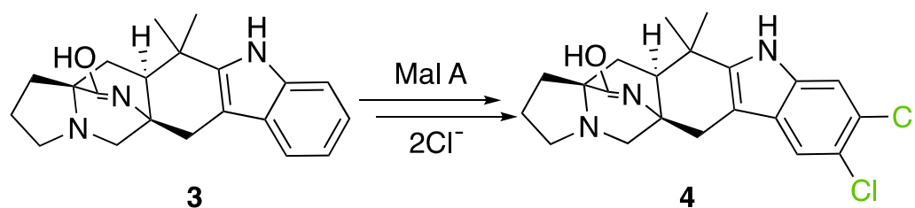
Figure 11. Premalbrancheamide (3) chlorination by MalA to obtain malbrancheamide (4).
