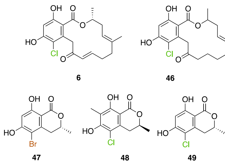
Figure 25. Structures of the metabolites found in the pochonin D cluster 1: pochonin D (6), monorden E (46), palmerin D (47), chaetosemin G (48), and 5-chloro-6-hydroxymellein (49).
