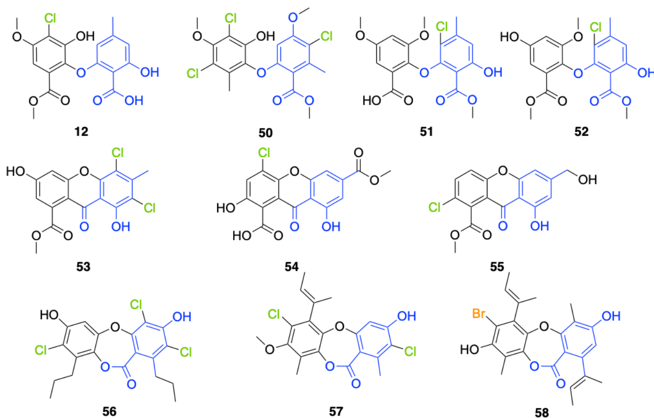
Figure 26. Pestheic acid (12) is included in cluster 2 containing buellin (50) from Diploicia sp.; chrysine D (51), penicillither (52), and penicillixanthone (53) from Penicillium sp.; 4-chlorocurvularinic acid (54) from Curvularia sp.; engyodontiumone B (55) from Engyodontium sp.; spiromastixone N (56) from Spiromastix sp.; aspersidone (57) from Aspergillus sp.; and 7-bromofolipastatin (58) from Aspergillus sp.
