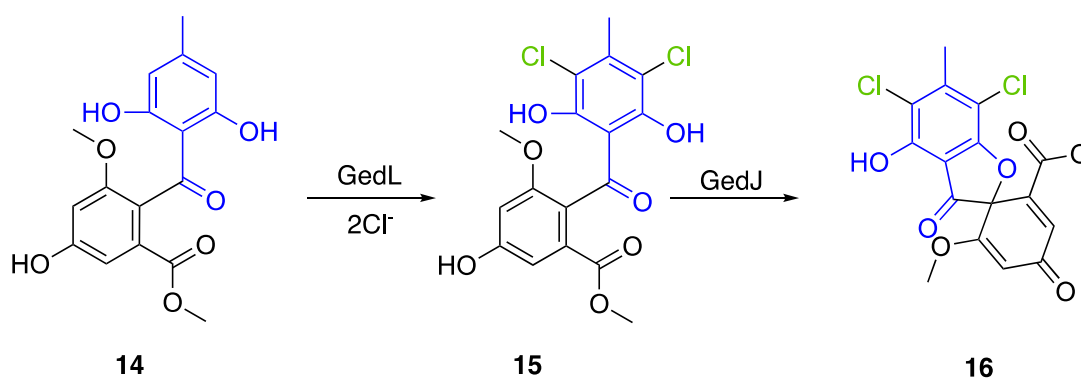
Figure 15. Dichlorination of sulochrin (14) by GedL in A. terreus to form dihydrogeodin (15) in the biosynthesis of geodin (16).
