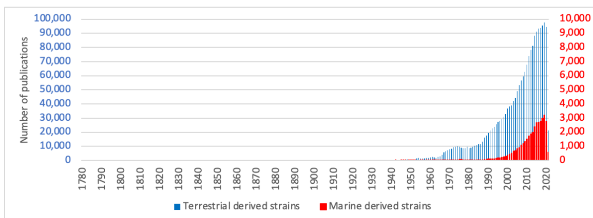
Figure 2. Evolution of the number of publications available on PubMed for terrestrial fungi (blue) and marine fungi (red) over the years (keywords used for PubMed research: (blue) “fungi” NOT “marine”, (red) “fungi” AND “marine”; “fungi” NOT “marine” excludes marine fungi from the research while “fungi” AND “marine” only selects strains from marine environment).
