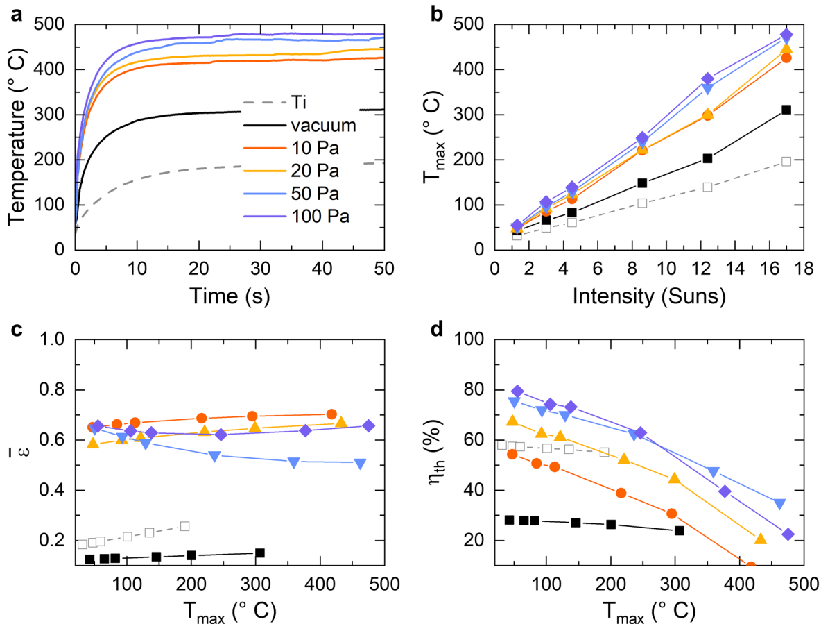
Figure 5. Solar-thermal performance of the investigated films. (a) Temperature profiles under 17 Suns as a function of time. (b) Maximum temperature (steady-state value at the end of each experiment) measured as a function of the solar power (1.3–17 Suns). (c) Spectrally averaged emittance and (d) thermal transfer efficiency as a function of the maximum temperature under irradiation. All panels report also the data for an uncoated titanium substrate.
