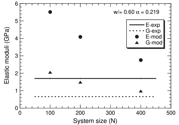
Fig. 7. Elastic moduli of cement paste system (w/c=0.60, \alpha=0.219 ) for the L cement, plotted against the number of voxels per 100 \mu\text{m} in the model. The straight lines are the experimental values, and the points are from numerical computations.
