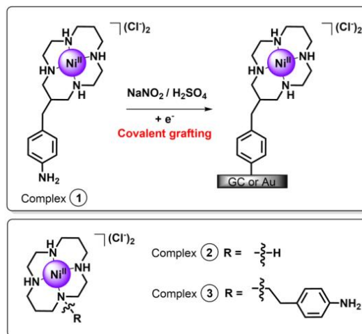
Scheme 1 Covalent grafting of complex 1 onto Au or GC electrode (top) and chemical representation of complexes 2 and 3 (bottom).
