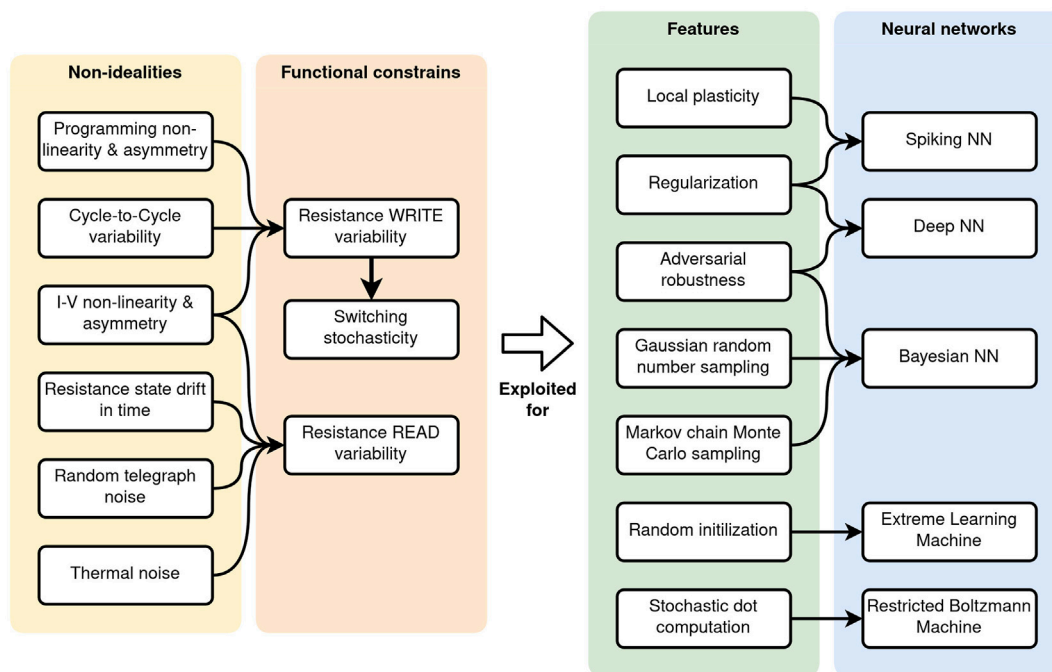
FIGURE 1 | Device-level non-idealities influence on RSM functional constraints and their possible usage for different NN architectures. The list of non-idealities and functional constraints given here is limited to those reported in the literature for these use cases, thus the list is not exhaustive.
