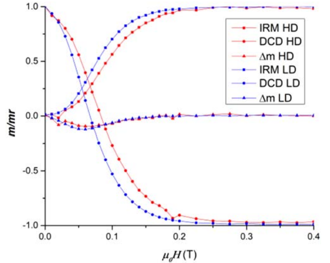
Fig. 8. IRM/DcD and \Delta m curves measured at 2 K on annealed LD and HD FeRh@C samples.
