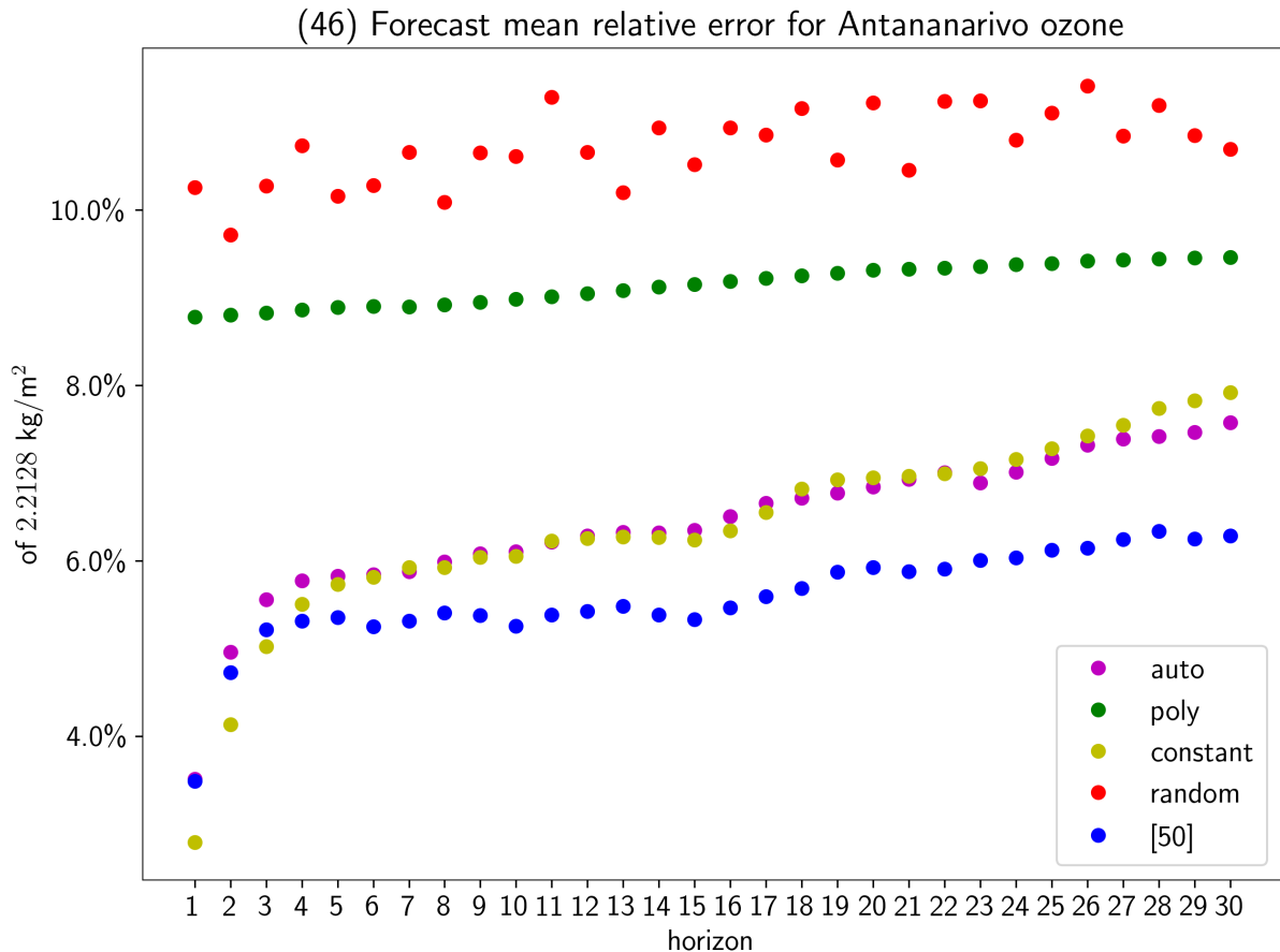
Figure 6: Forecast mean relative error for Antananarivo ozone
