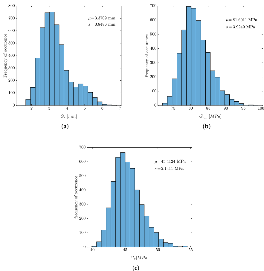
Figure 11. Statistical distribution of the vertical irregularity and stresses random variables. (a) Vertical irregularity variable G_r . (b) Normal stress variable G_{\sigma_{xx}} . (c) Shear stress variable G_{\tau} .
