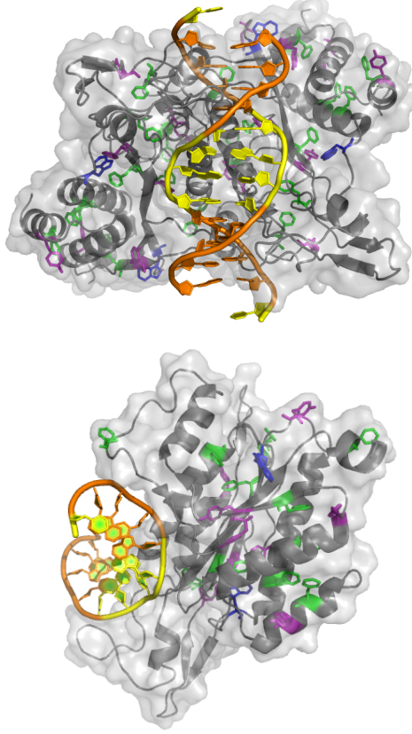
Figure 7: Aromatic network in EcoRI -DNA complex. Tryptophan (blue), tyrosine (purple), and phenylalanine (green) form correlated electronic dispersion networks in EcoRI , shown here in the top panel bound to its double-stranded DNA substrate, with adenine-thymine (yellow) and cytosine-guanine (orange) base pairs highlighted. Other amino acids (gray) are displayed in the context of their secondary structures within the enzyme, and in the bottom panel only one of the two EcoRI dimers is shown for clarity, to showcase the \pi - \pi stacking of the DNA bases. Image of EcoRI (PDB ID: 1CKQ) at 1.85 Å resolution created with PyMOL and adapted from [18].
