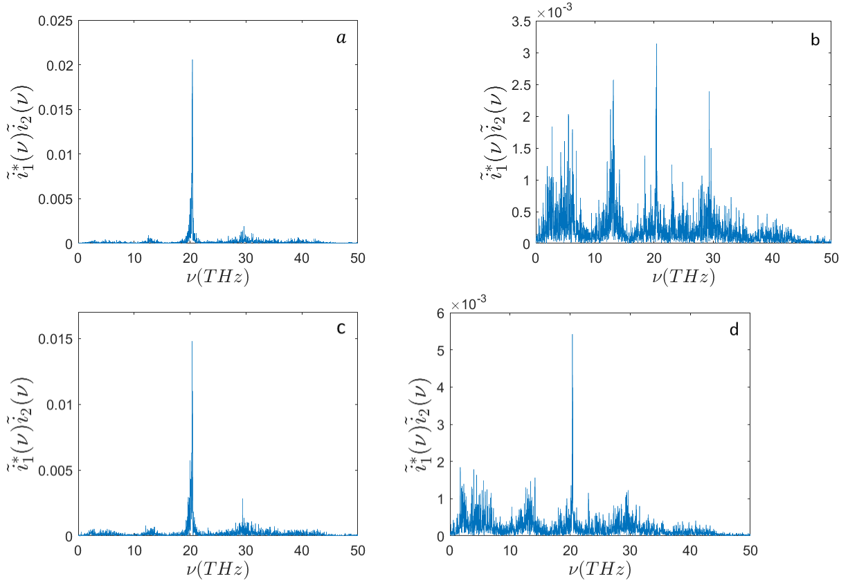
Figure 3: The cross frequency spectrum of the interaction between DNA strand with N_1 = 66 nucleotides and the EcoRI enzyme with N_2 = 276 amino acids for the initial conditions: T = 310^\circ K , N_{0,1} = N/2 , N_{0,2} = N/3 , E'_{1,0} = 110 , E'_{2,0} = 30 , \epsilon'_1 = \epsilon'_2 = 5 , \mu'_1 = \mu'_2 = 0.5 , \Omega'_2 = 0.79 and site-dependent parameters \Omega_{1,n} = 0.48/m_n , J'_{1,n} , J'_{2,n} , \chi'_{1,n} and \chi'_{2,n} corresponding to E_{0,1} = 0.72 eV, E_{0,2} = 0.2 eV, \epsilon_1 = \epsilon_2 = 0.0329 eV, \mu_1 = \mu_2 = 0.5 , \Omega_{2,n} = V^2\langle M \rangle/a^2 , \Omega_{1,n} = V^2M_n/a^2 , J_{1,n} , J_{2,n} , \chi_{1,n} and \chi_{2,n} regarding to the Equations (15) and (16); and \sigma_{1,0} = \sigma_{2,0} = 0.1 . a) DNA containing the specific CTTAAG recognition sites, b) randomized restriction sites AGCTTA, c) exchanging only one nucleotide with its complementary CATAAG, d) exchanging two nucleotides with their complementaries GTTAAC.
