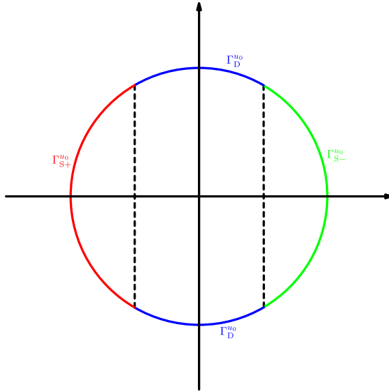
FIGURE 1. Boundary decomposition for the two-dimensional example of Section 4.
