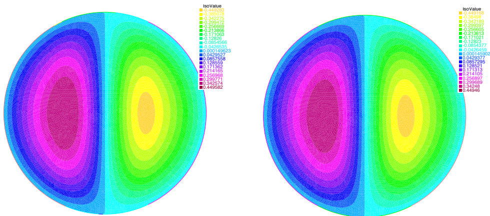
FIGURE 3. Case t = 0.01 ( d = 2 ): solution u_t (left) and its first-order approximation u_0 + tu'_0 (right).
