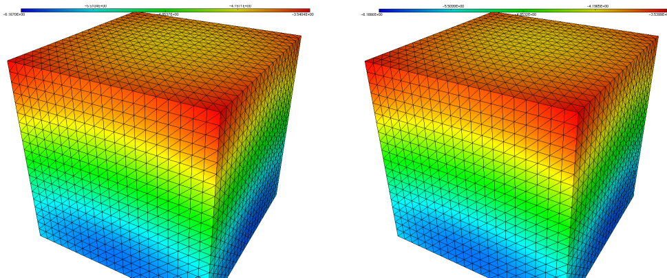
FIGURE 4. Case t = 0.1 ( d = 3 ): solution u_t (left) and its first-order approximation u_0 + tu'_0 (right).
