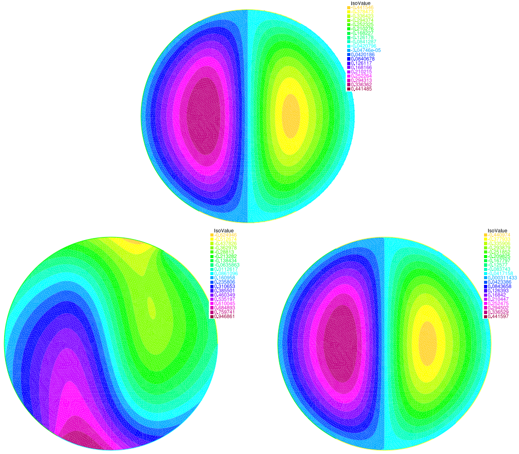
FIGURE C.1. Resolution of a Tresca-type problem: exact solution ( top ), initial solution ( bottom left ) and approximated solution ( bottom right ).
