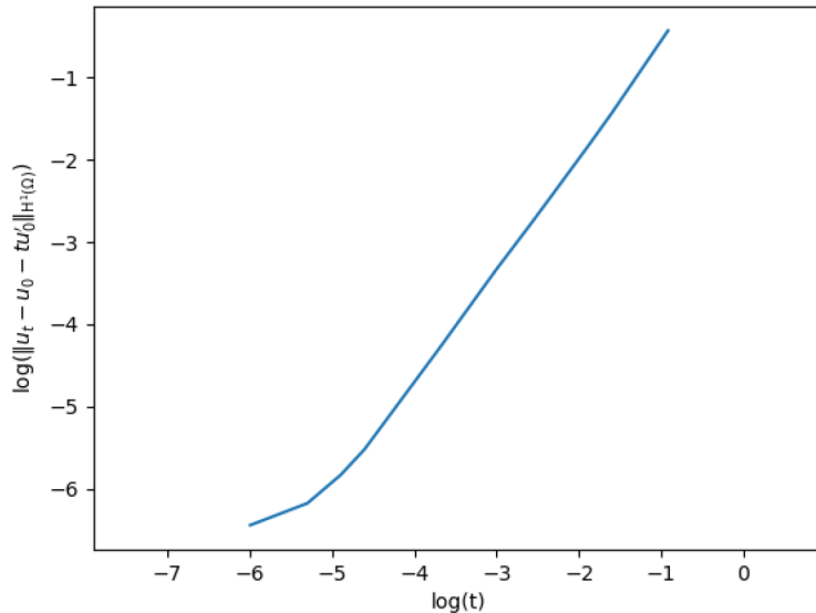
FIGURE 2. The H^1 -comparison \|u_t - u_0 - tu'_0\|_{H^1(\Omega)} with respect to t in logarithmic scale.
