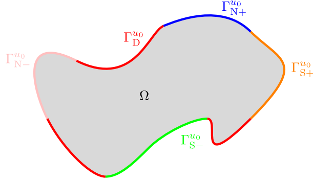
FIGURE B.1. Illustration on an admissible decomposition of \Gamma .
