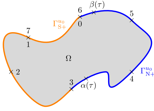
FIGURE B.2. Illustration of the parameterization (B.1) of \Gamma .
