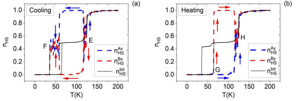
FIG. 10. Thermal-dependence of HS fractions, n_{HS}^A (blue dashed curve) and n_{HS}^B (red dashed curve) of the two sublattices, A and B, constituted of alternate stripes in the coexistence region of the plateau, during cooling (a) and heating (b) and the total HS fraction, n_{HS}^{tot} (black curve), for B = 2 \cdot 10^4 \text{ K} \times \text{nm}^{-2} and A = 100 \text{ K} \times \text{nm}^{-2} . The black continuous line is the total HS fraction. The alternate stripes are along x-direction (y-direction) on cooling (resp. heating) and are characterized by their order parameter n_{HS}^{A,m} and n_{HS}^{B,m} where m = x, y , denotes the direction of the stripes. Clear symmetry breaking appear at point E on cooling and point G on heating.
