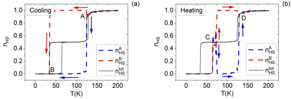
FIG. 4. Thermal-dependence of HS fractions, n_{HS}^A (blue dashed curve) and n_{HS}^B (red dashed curve) of the two sublattices, A and B, in the coexistence region of the plateau, on cooling (a) and on heating (b) and the total HS fraction, n_{HS}^{tot} (black curve), for A = 40000 \text{ K} \times \text{nm}^{-2} and B = 100 \text{ K} \times \text{nm}^{-2} . The black continuous line is the total HS fraction. The bifurcations of the sublattices order parameters, n_{HS}^A and n_{HS}^B at points A and B (resp. C and D) on cooling (heating) announces the presence of a symmetry breaking between A and B sublattices.
