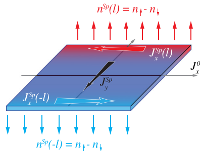
FIG. 2. Superimposition of the two channels represented for the symmetric device and environment ( C_E = 0 in the text). The electric generator and the injected current J_x^0 are not shown for clarity. The system is characterized by the absence of the total charge accumulation, the spin accumulation n^{sp}(y) = \delta n_{\uparrow}(y) - \delta n_{\downarrow}(y) with opposite directions at the two edges, the inhomogeneous part of the longitudinal spin currents J_x^{sp}(y) = J_{x\uparrow}(y) - J_{x\downarrow}(y) , and the transverse spin current J_y^{sp} = J_{y\uparrow}(y) - J_{y\downarrow}(y) .
