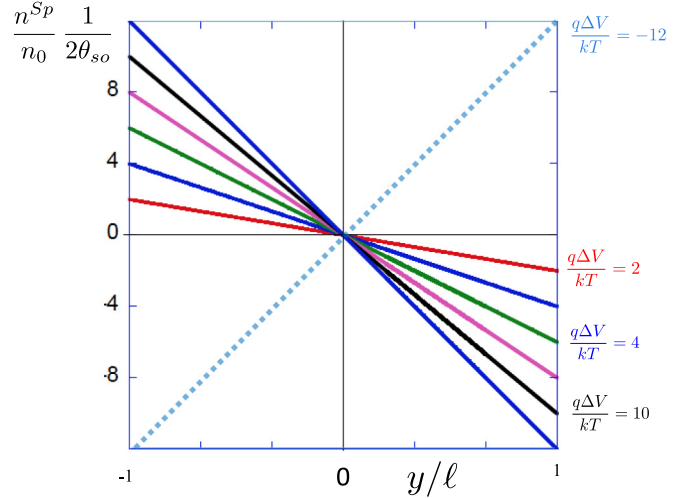
FIG. 4. Spin accumulation n^{Sp} [Eq. (20) in the text] as a function the ratio y/\ell for different values of the ratio q\Delta V/kT , from q\Delta V/kT = 2 to q\Delta V/kT = 12 . The spin accumulation is normalized by the product of the density of carriers at equilibrium 2n_0 by the spin Hall angle \theta_{so} . The curve for q\Delta V/kT = -12 shows that reversing the electric polarity reverses the sign of the spin accumulation.
