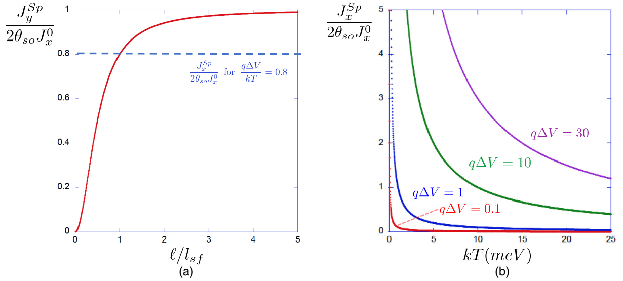
FIG. 3. (a) Transverse pure spin current J_y^{Sp} [Eq. (37) in the text] as a function the ratio \ell/l_{sf} of the width of the spin Hall bar over the spin-flip scattering length [Eq. (37) and Eq. (36)]. (b) Longitudinal pure spin current J_x^{Sp} as a function of the temperature [Eq. (39)] and [Eq. (20)] for different values of the injected voltage q\Delta V , expressed in meV . The amplitude is calculated for y = L = \ell . The currents are normalized by the product of the injected current 2J_x^0 by the spin Hall angle \theta_{so} at the first order in \theta_{so} .
