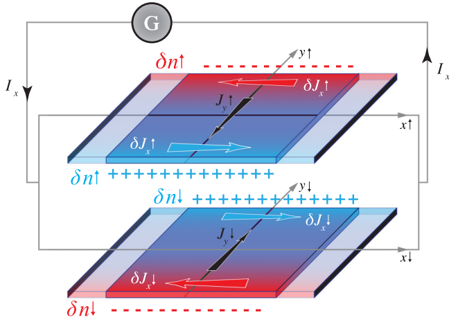
FIG. 1. Schematic representation of the two channel model (corresponding to spin \uparrow and spin \downarrow ) for a spin Hall bar. The device is contacted to an electric generator that imposes a longitudinal stationary current J_x^0 (not shown). The charge accumulations \pm\delta n_{\uparrow\downarrow} and the inhomogeneous part of the longitudinal currents \delta J_{x\uparrow\downarrow}(y) = J_{x\uparrow\downarrow}(y) - J_x^0 are represented at both edges for each channel together with the transverse current J_{y\uparrow\downarrow} flowing from one edge to the other.
